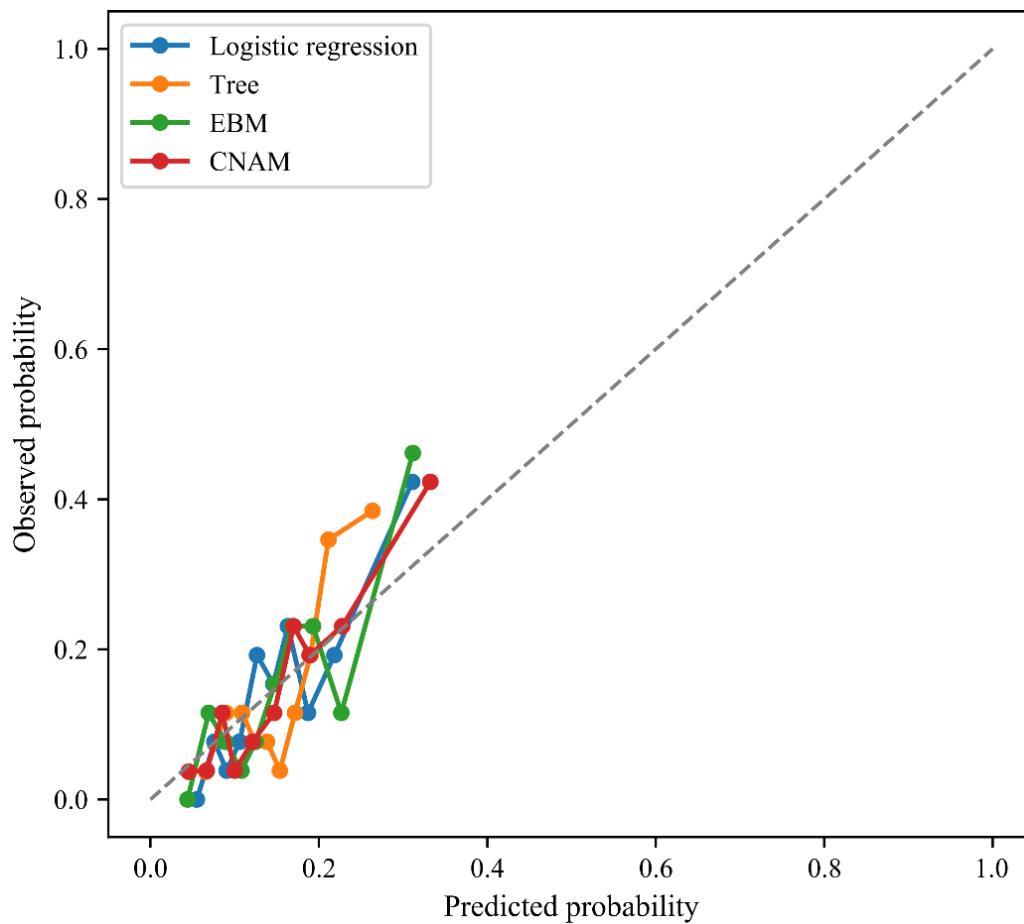
Figure 4. Calibration curves on the locked test set after sigmoid calibration fitted on development out-of-fold predictions. Post hoc calibration improved probability reliability, especially for CNAM.
