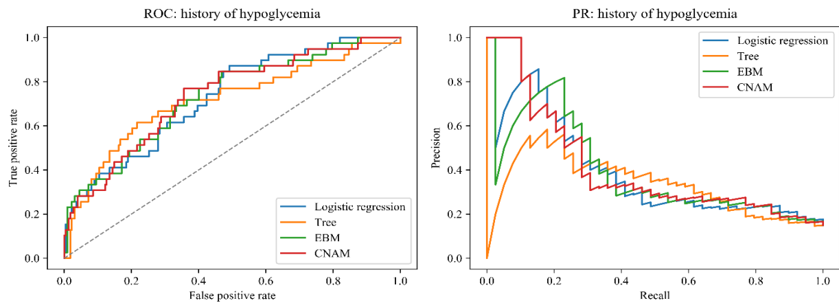
Figure 3. Receiver operating characteristic (ROC) and precision–recall (PR) curves on the locked test set for logistic regression, gradient-boosted trees, explainable boosting machine (EBM), and the proposed knowledge-constrained neural additive model (CNAM)
