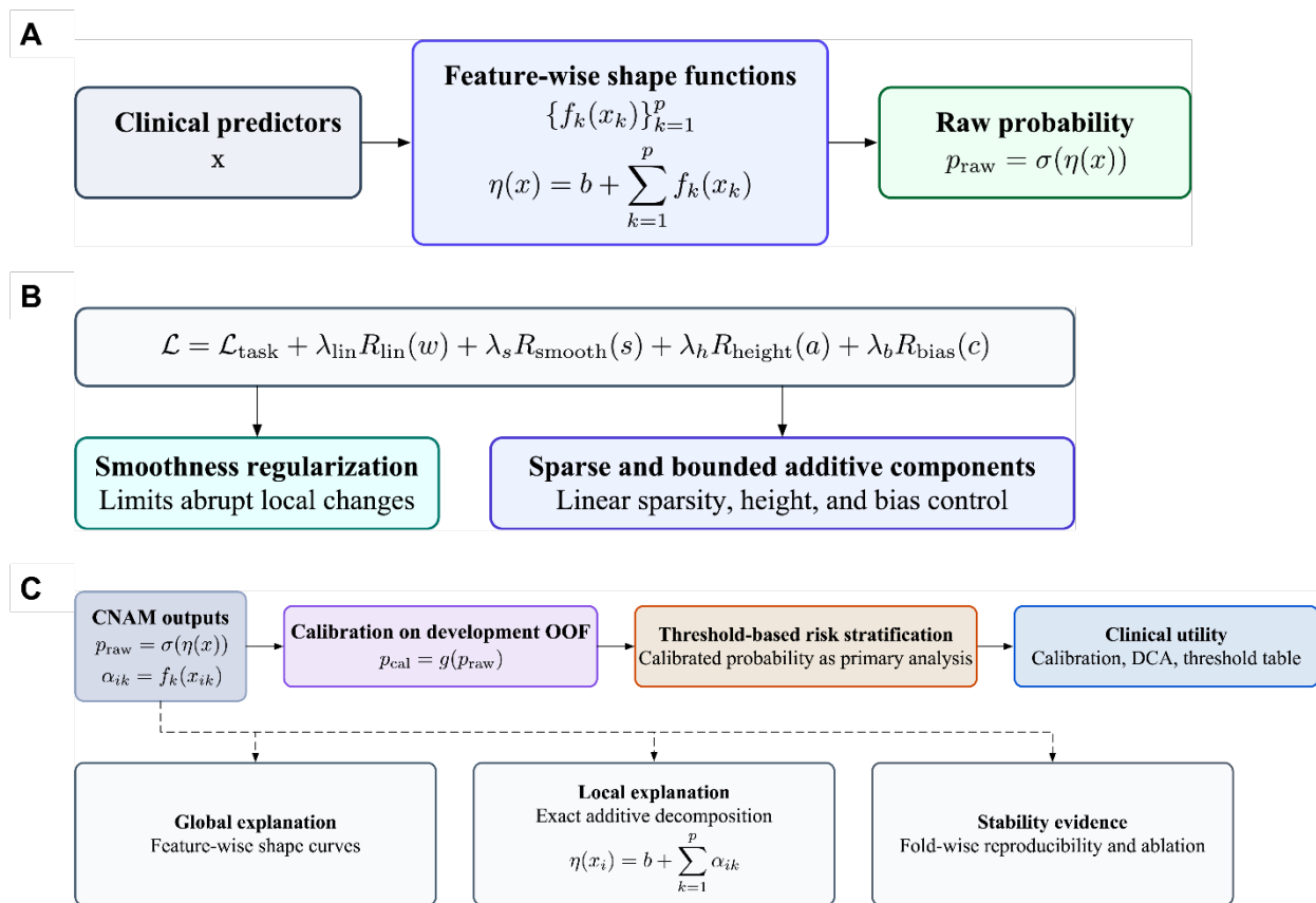
Figure 2. Detailed schematic view of the proposed knowledge-constrained neural additive model (CNAM) modeling framework. (A) Step-based additive representation from clinical predictors to the additive logit and raw probability. (B) Knowledge-guided learning through a constrained objective with linear sparsity, smoothness, amplitude, and bias penalties. (C) Compact decision-support-oriented summary of calibrated decision support and structural explanation.
