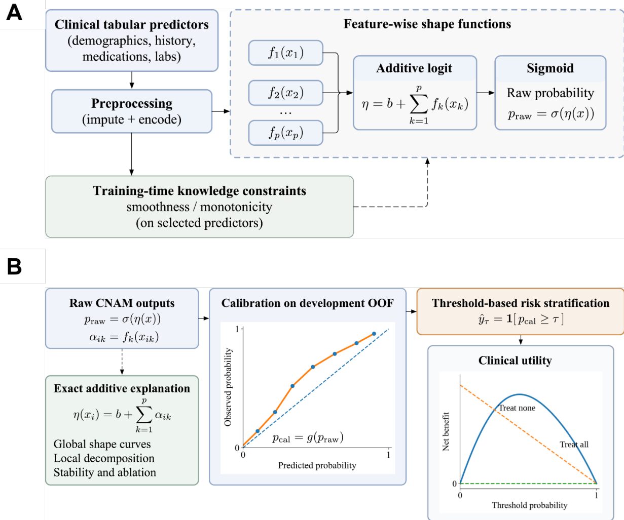
Figure 1. Framework-level overview of the proposed knowledge-constrained neural additive model (CNAM). (A) Training-time additive modeling from clinical tabular predictors to the raw probability, with smoothness and monotonicity constraints applied to feature-wise shape-function learning. (B) Decision-support-oriented outputs of the framework, including probability calibration, threshold-based risk stratification, clinical utility analysis, and exact additive explanations.
