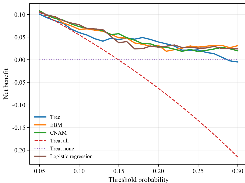
Figure 5. Decision curve analysis on the locked test set. CNAM and logistic regression had broadly similar net-benefit profiles across the evaluated threshold range, and calibrated CNAM retained positive net benefit across clinically relevant threshold probabilities. Abbreviations: CNAM: Knowledge-constrained neural additive model; EBM: Explainable boosting machine.
