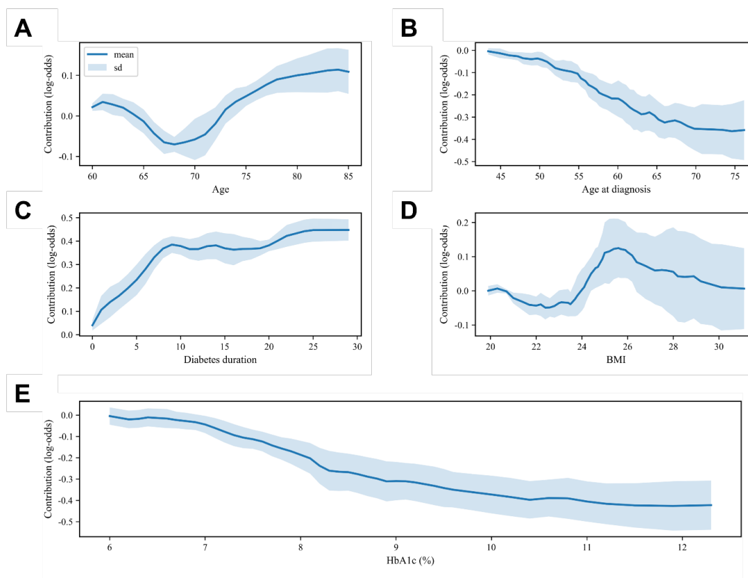
Figure 6. Stability of knowledge-constrained neural additive model (CNAM) shape functions across outer folds for key continuous predictors. (A) Age. (B) Age at diagnosis. (C) Diabetes duration. (D) Body mass index (BMI). (E) Glycated hemoglobin (HbA1c). The most clinically salient feature effects remained reproducible across repeated model fits.
