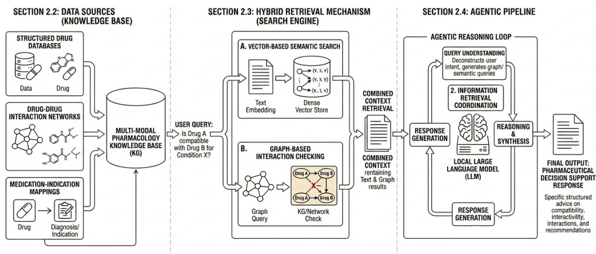
Figure 1. Graph-Enhanced Retrieval-Augmented Generation (Graph-Enhanced RAG) system for pharmaceutical decision support
