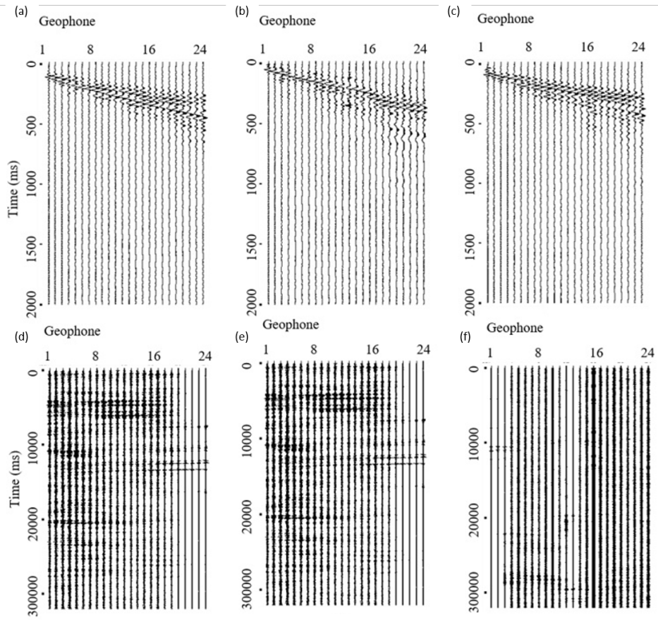
Figure 5. Active-source seismograms (a–c) and roadside-passive seismograms (d–f) at Sites 1–3
