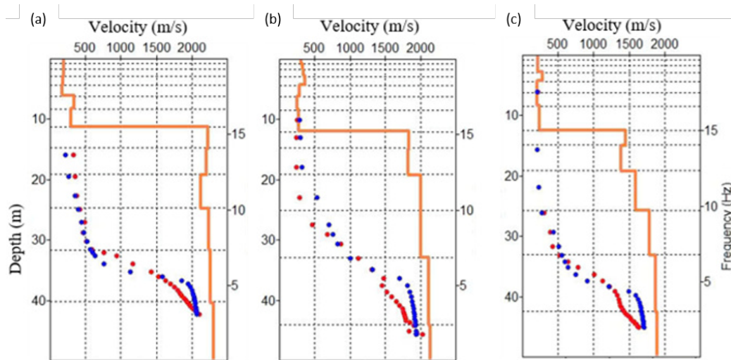
Figure 9. Final one-dimensional V_s profiles at Sites 1–3; blue and red points denote observed (picked) and calculated dispersion, respectively
