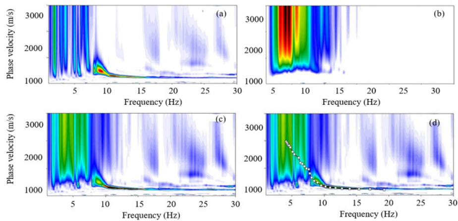
Figure 7. Site 2: (a) active dispersion image, (b) passive dispersion image, (c) combined image, and (d) combined image with manually picked fundamental-mode curve
