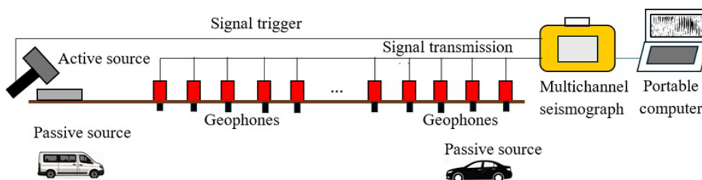
Figure 3. Co-located configurations for active-source and roadside-passive multichannel analysis of surface waves acquisition
