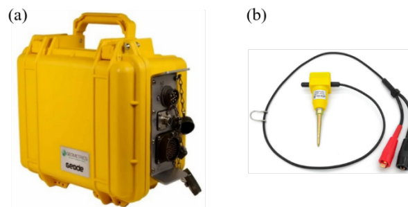
Figure 4. Field equipment: (a) 24-channel GEODE seismograph and (b) 4.5-Hz vertical geophone
