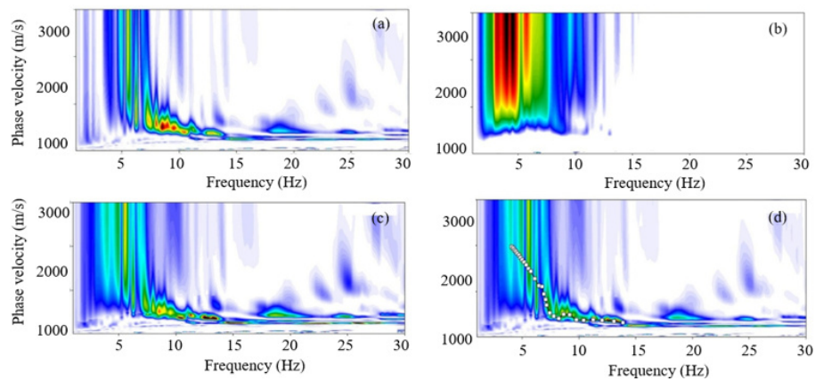
Figure 6. Site 1: (a) active dispersion image, (b) passive dispersion image, (c) combined image, and (d) combined image with manually picked fundamental-mode curve
