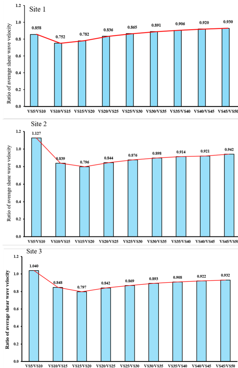
Figure 11. Successive 5-m ratios of depth-averaged shear-wave velocity at Sites 1–3. Labels such as VS10/VS15 denote VS,10/VS,15 and represent the 10–15 m depth interval.
