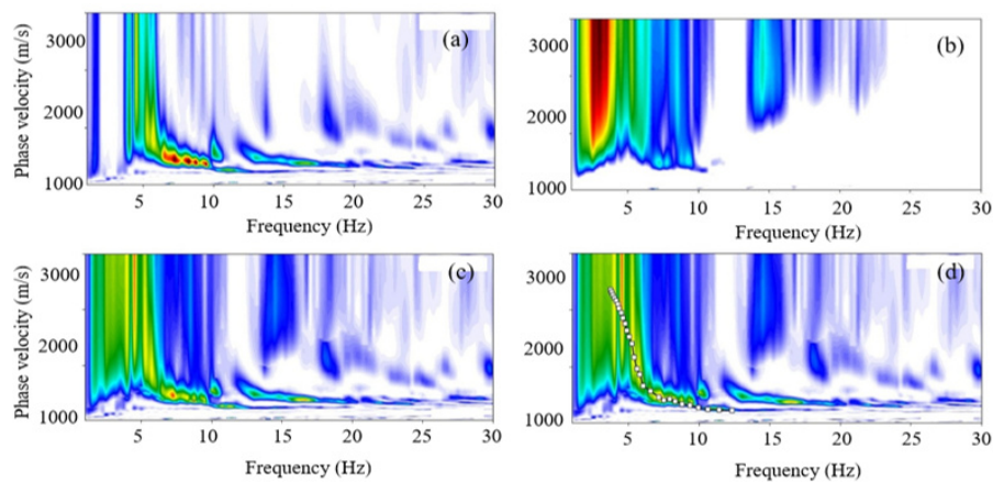
Figure 8. Site 3: (a) active dispersion image, (b) passive dispersion image, (c) combined image, and (d) combined image with manually picked fundamental-mode curve
