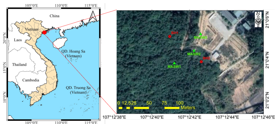
Figure 1. Locations of the three co-located active-passive multichannel analysis of surface waves lines and two geological boreholes in Quang Hanh Ward
