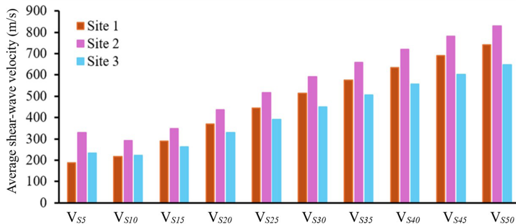
Figure 10. Depth-averaged shear-wave velocity from the surface to 5–50 m at Sites 1–3
