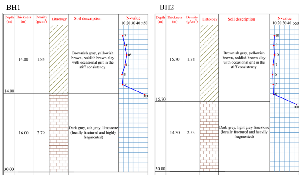
Figure 2. Borehole lithology and Standard Penetration Test results used to validate the interpreted stiffness boundary
