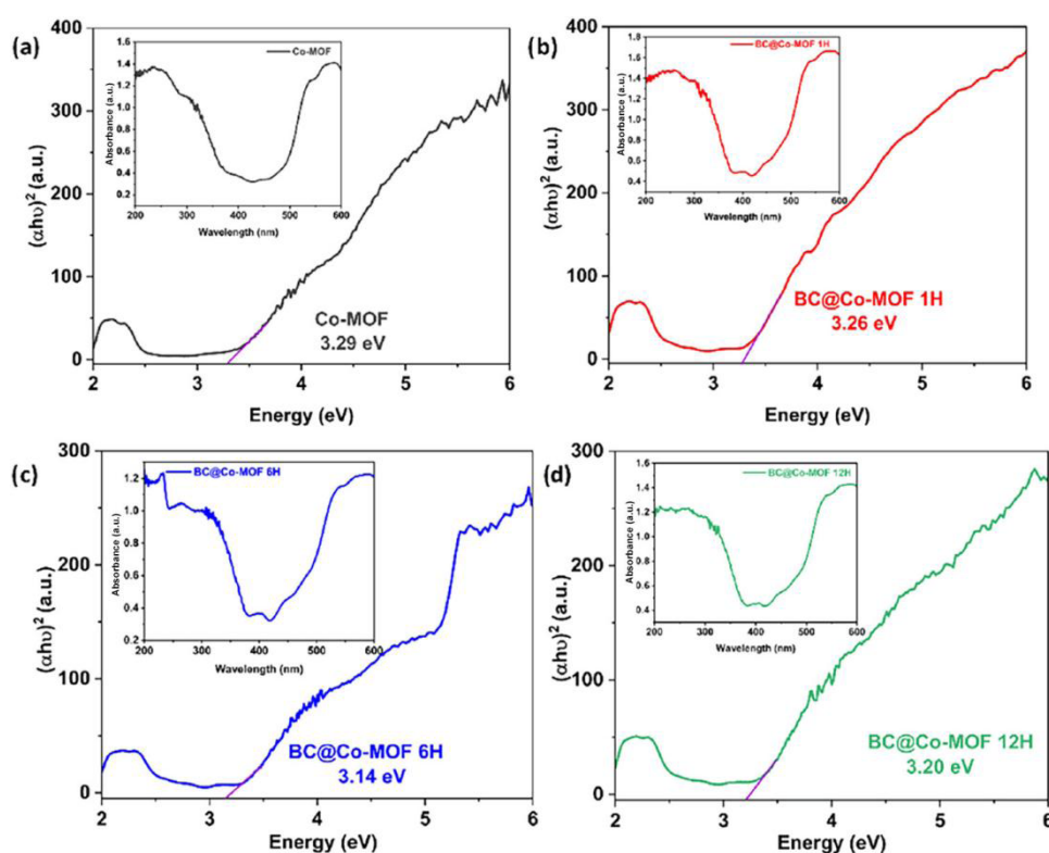
Figure 2. Ultraviolet-diffuse reflectance spectroscopy spectra and Tauc plot of (A) Co-MOF, (B) BC@Co-MOF 1H, (C) BC@Co-MOF 6H, and (D) BC@Co-MOF 12H 45
