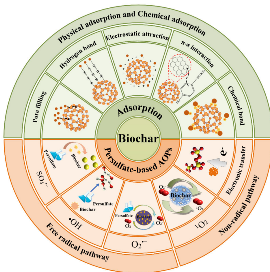
Figure 3. Removal mechanisms and main interactions of pharmaceutical pollutants by biochar 52
