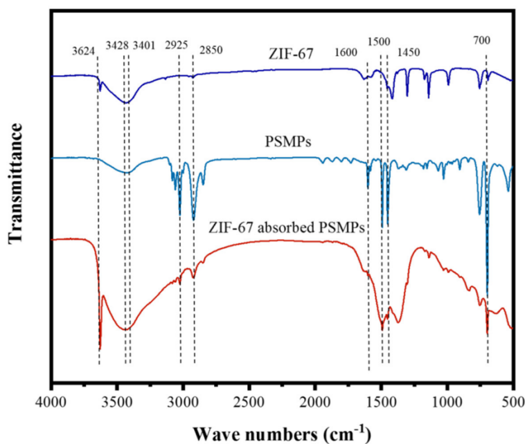
Figure 4. Fourier-transform infrared spectroscopy spectra for PSMPs and ZIF-67 during the adsorption process 59 Abbreviations: PSMPs: Polystyrene microplastics; ZIF: Zeolitic imidazolate framework.
