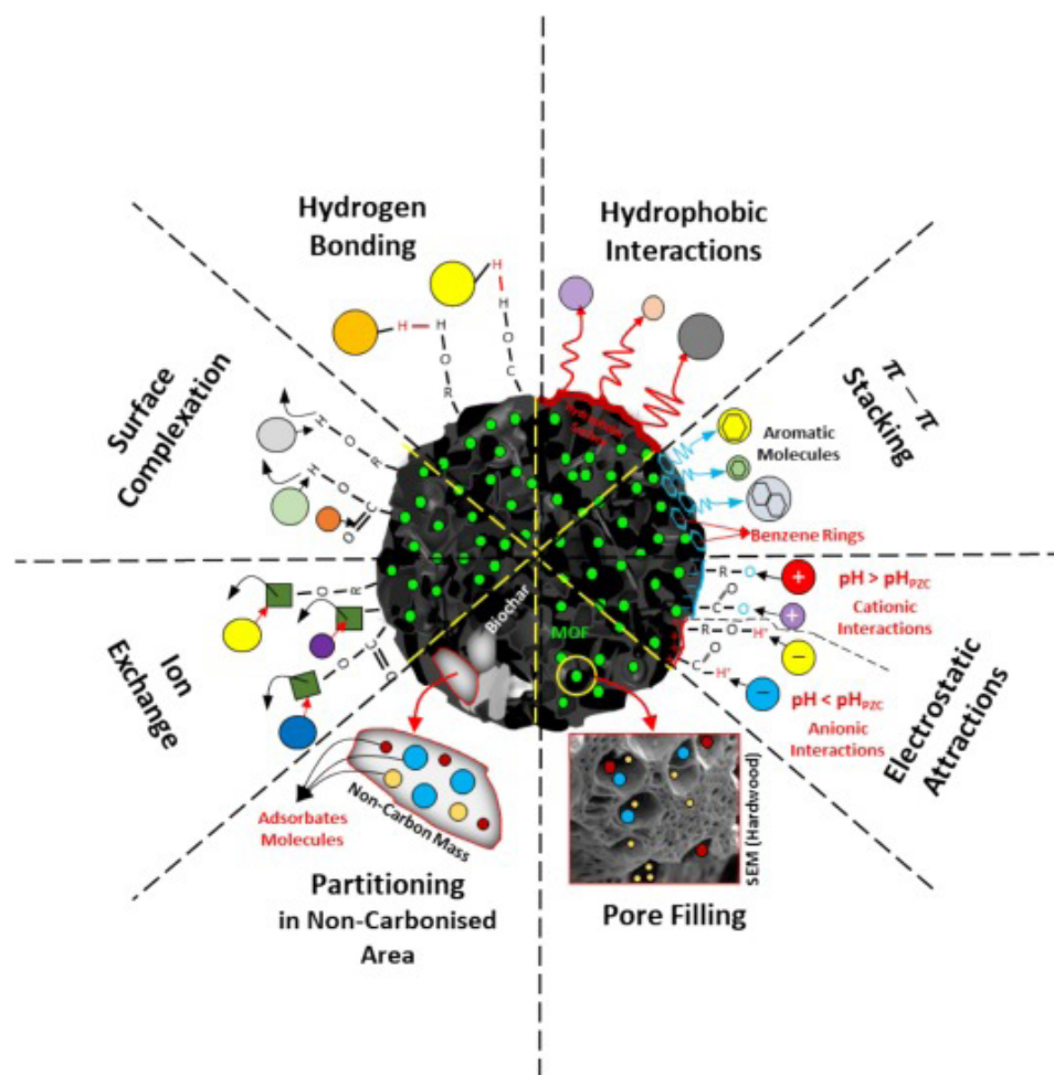
Figure 1. Schematic illustration of possible adsorption mechanisms in metal-organic framework-biochar composites 25 Abbreviations: MOF: Metal-organic framework; SEM: Scanning electron microscopy.
