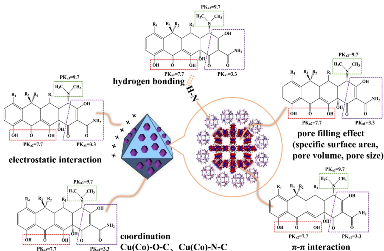
Figure 5. The adsorption mechanism of tetracyclines on Cu-MOF@Co-MOF 71 Abbreviation: MOF: Metal-organic framework.
