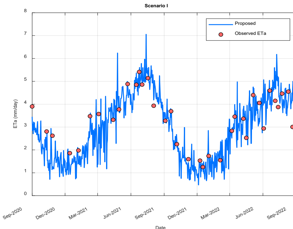
Figure 6. Temporal variation of model results for Scenario I, illustrating the seasonal stability and general agreement of predicted ETa with observations
