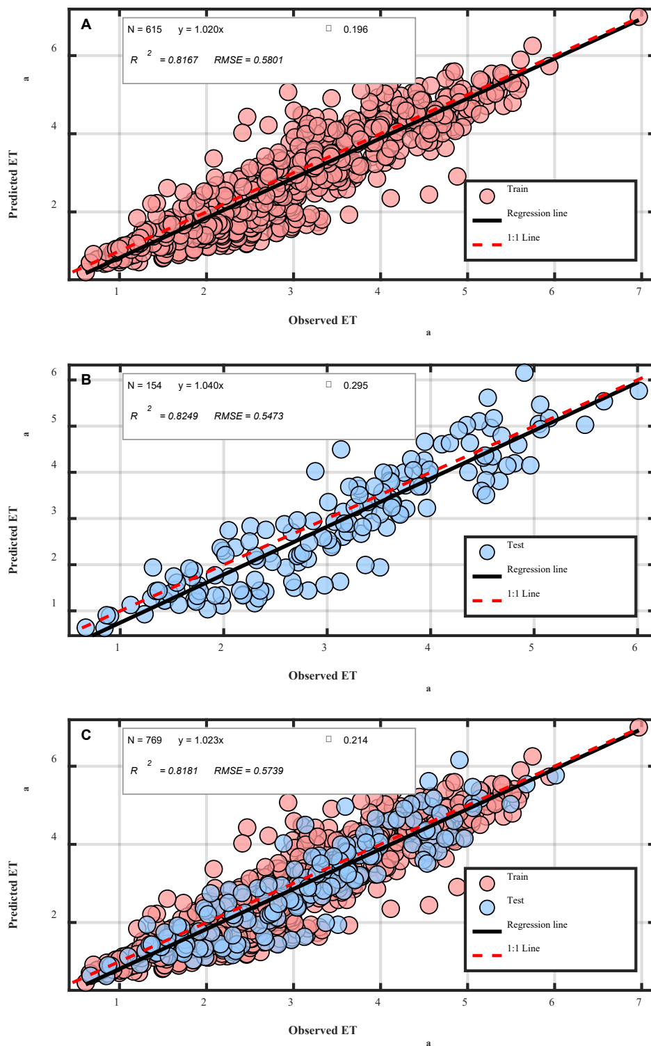
Figure 7. Model results for Scenario II, showing the comparison between observed and predicted ETa values for (A) training, (B) test, and (C) full datasets
