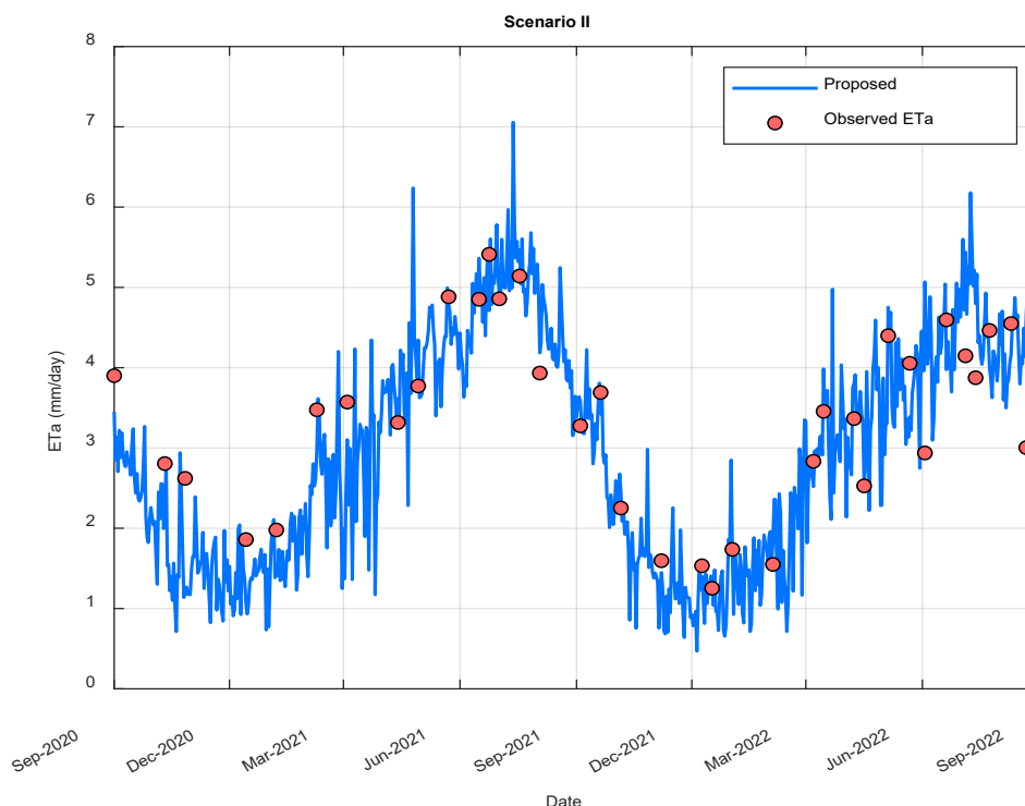
Figure 8. Temporal variation of model results for Scenario II, demonstrating the consistent alignment of predicted and observed ETa values throughout the study period
