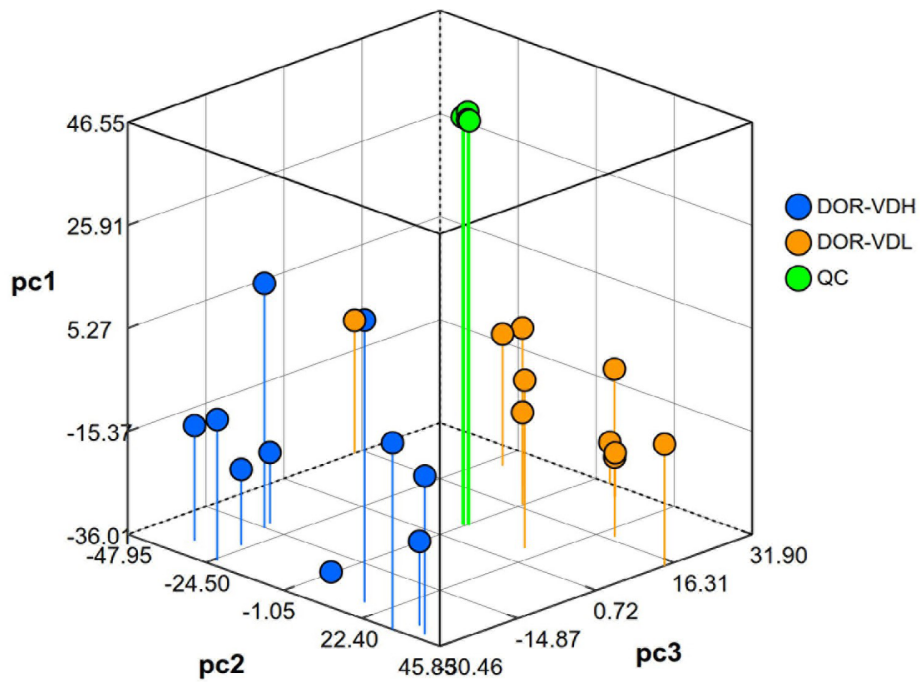
Figure S2. Three-dimensional principal component analysis of the DOR subgroups Abbreviations: DOR: Diminished ovarian reserve; QC: Quality control; VDH: Vitamin D non-deficient; VDL: Vitamin D deficient.
