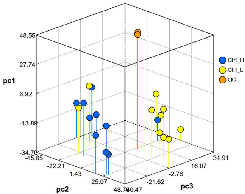
Figure S3. Three-dimensional principal component analysis of the control subgroups Abbreviations: QC: Quality control; VDH: Vitamin D non-deficient; VDL: Vitamin D deficient.
