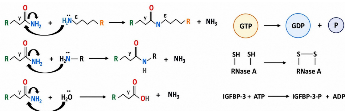
Figure 2. Reactions catalyzed by TG2. (I) Transamidation between the \gamma -carboxamide group of a glutamyl residue and the \epsilon -amino group of a lysyl residue; (II) transamidation between the \gamma -carboxamide group of a glutamyl residue and a polyamine; (III) deamination; (IV) GTPase activity; (V) protein disulfide isomerase activity; (VI) kinase activity.
