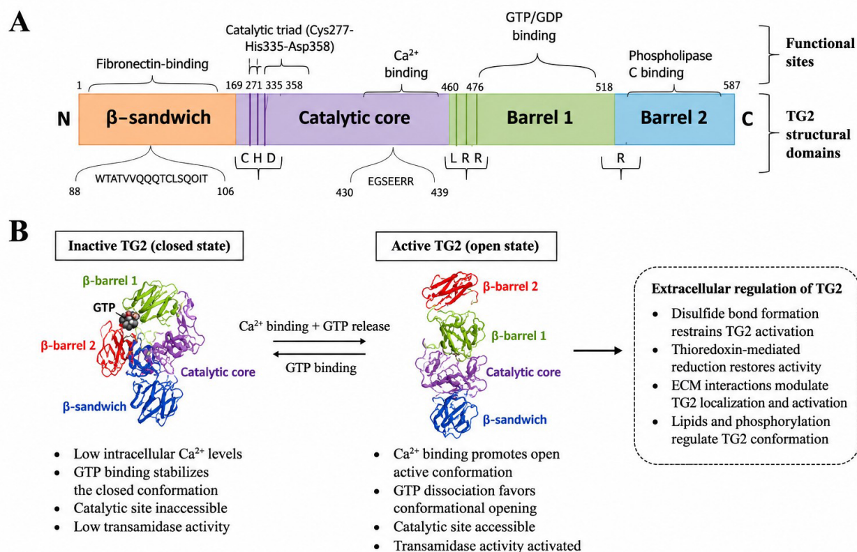
Figure 3. Schematic diagram of TG2 structure and functional domains. TG2 is composed of four domains. (A) The N-terminal \beta -sandwich mediates interactions with the ECM and contains binding sites for integrins and fibronectin. In its extended conformation, the catalytic core mediates protein polymerization and may contribute to apoptosis. (B) The \beta -barrel 1 domain contains the GTP/GDP-binding site and plays a key role in TG2-mediated signal transduction. The C-terminal \beta -barrel 2 domain, in the GTP-bound form, can recruit and activate phospholipase C and mediate pro-inflammatory functions.
