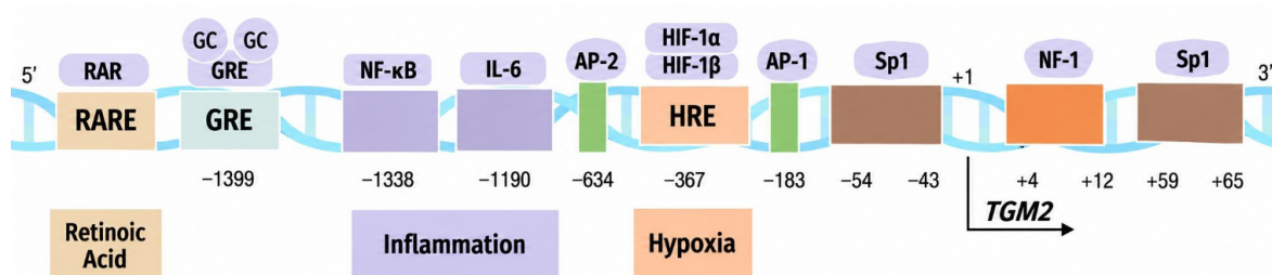
Figure 4. TGM2 promoter and its response elements. Response elements for RAR/RXR (–1,731 bp and –1,720 bp), glucocorticoid, (GRE; –1,399 bp), NF-κB (–1,338 bp), IL-6 (–1,190 bp), TGF-β1 (–900 bp), estrogen (ERE; –656 bp), AP-2 (–634 bp), HIF (HRE; –367 bp), AP-1 (–183 bp), and NF-1 (+4 bp, +12 bp), as well as motif regions such as CAAT box (–96 bp), TATA box (–29 bp), and GC box (Sp1, –54 bp, –43 bp, +59 bp, +65 bp) have been identified within the TGM2 promoter.
