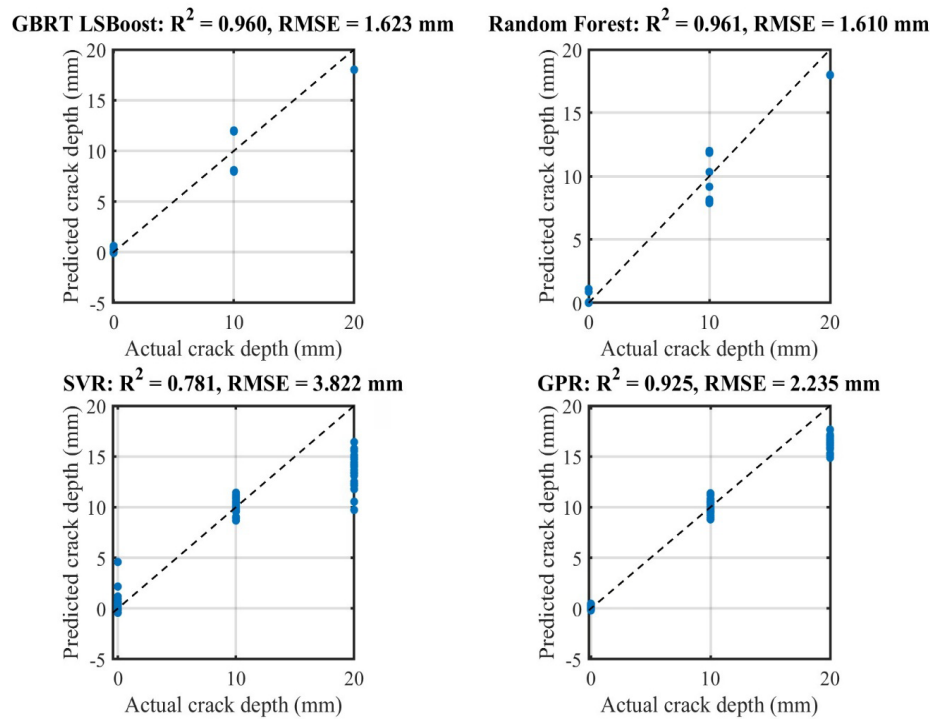
Figure 7. Crack depth prediction performance
