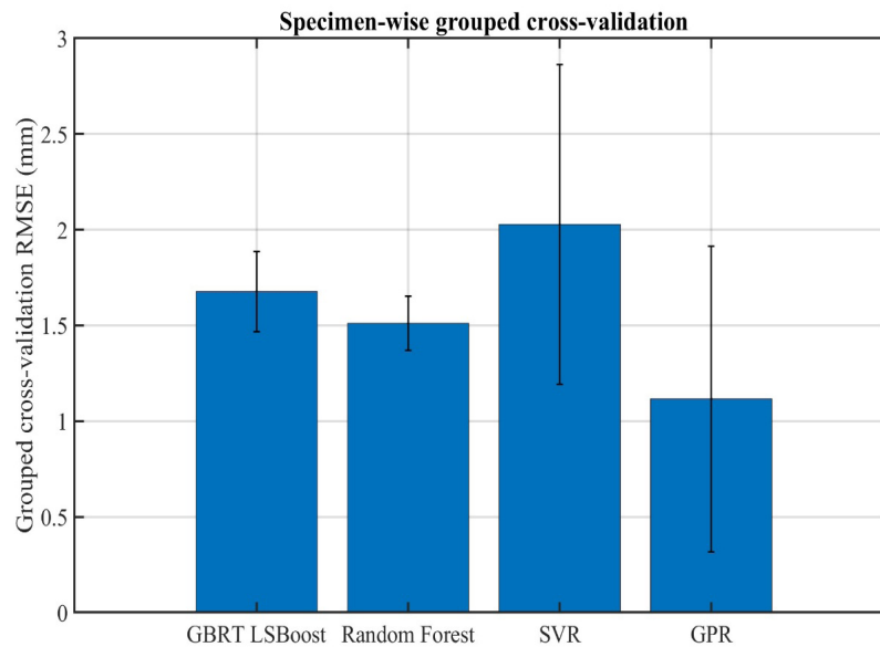
Figure 9. Specimen-wise grouped cross-validation results for the four ML regression models
