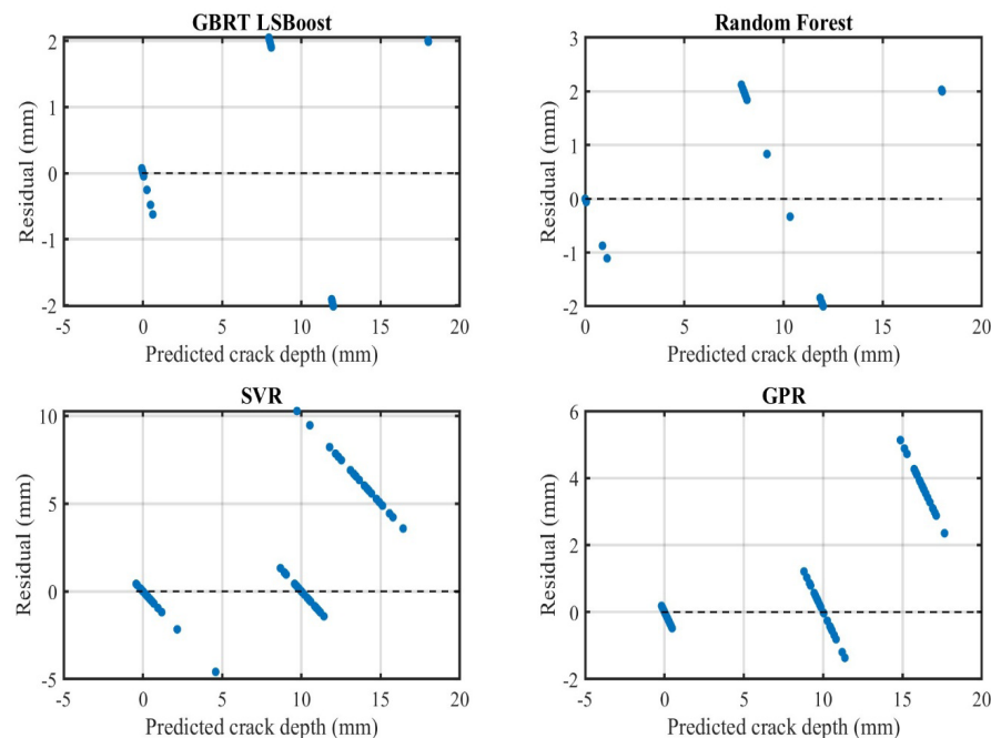
Figure 8. Residual distribution performance
