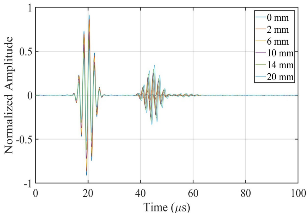
Figure 4. Time domain signals captured for different crack depths
