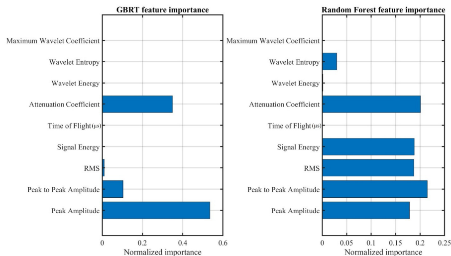
Figure 10. Feature importance from Gradient Boosted Regression Tree (GBRT)
