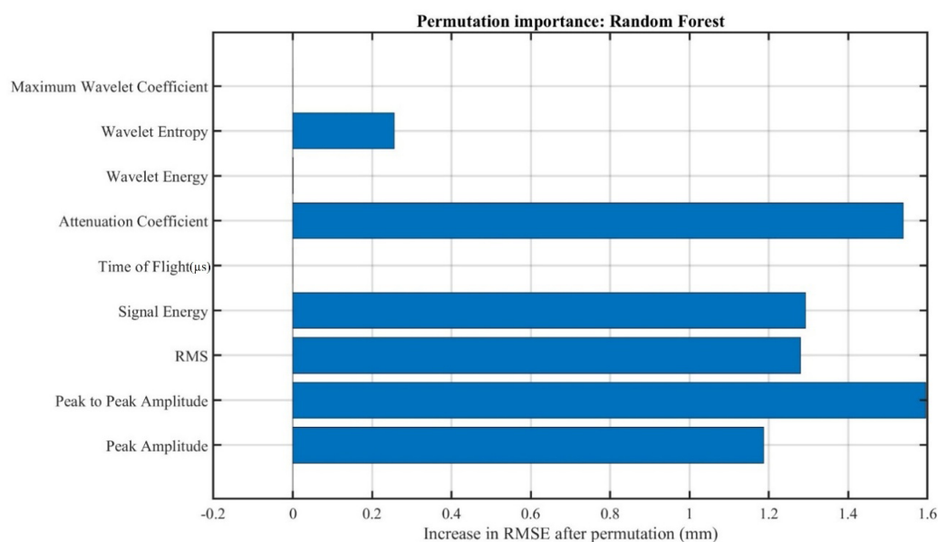
Figure 11. Permutation feature importance obtained using the Random Forest regression model
