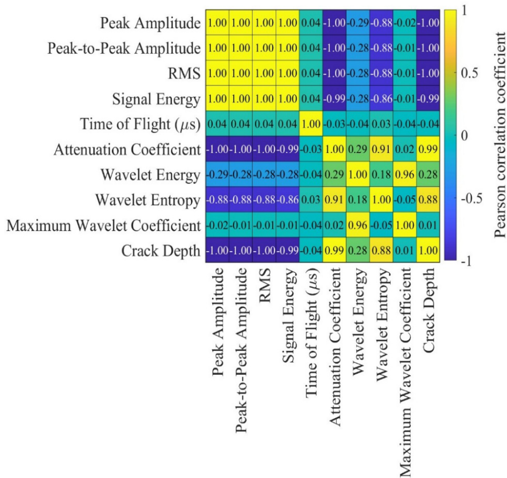
Figure 6. Pearson correlation matrix
