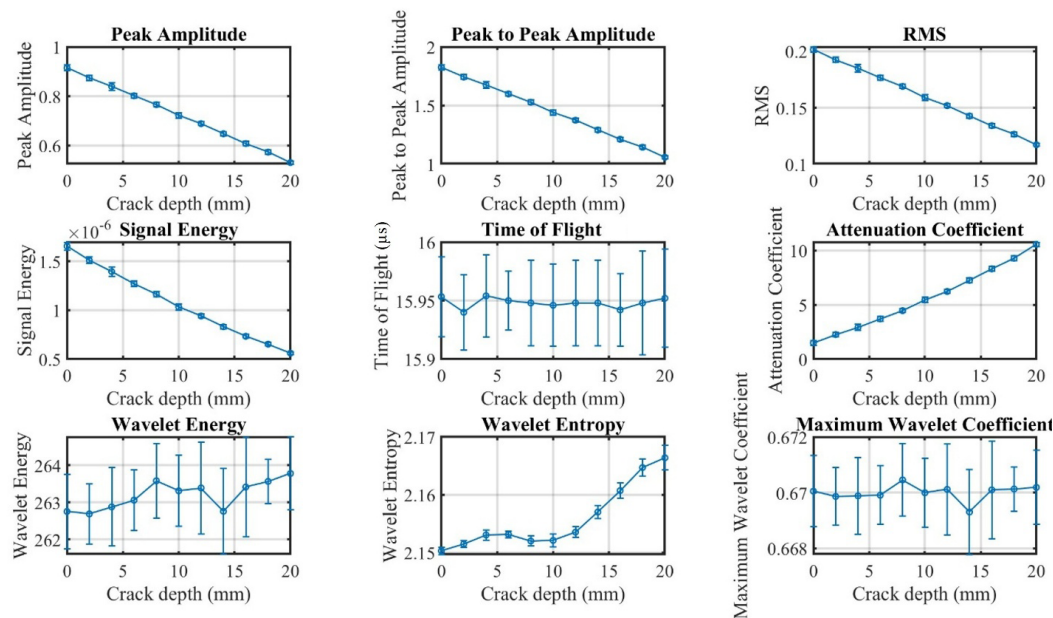
Figure 5. Variation of physics-based ultrasonic features with increasing crack depth
