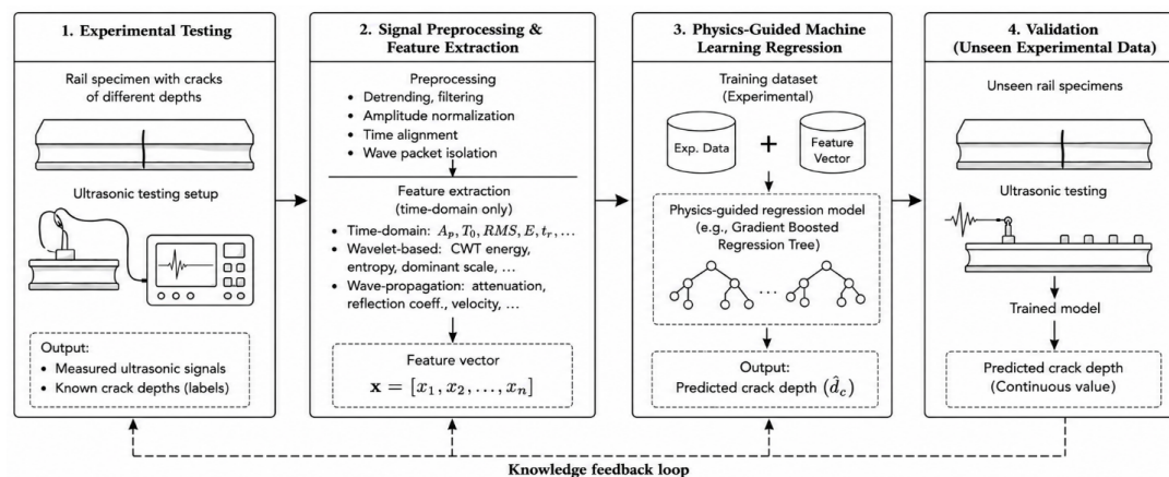
Figure 2. Overall workflow of the proposed physics guided wave machine learning framework for the crack depth quantification in rail track structures
