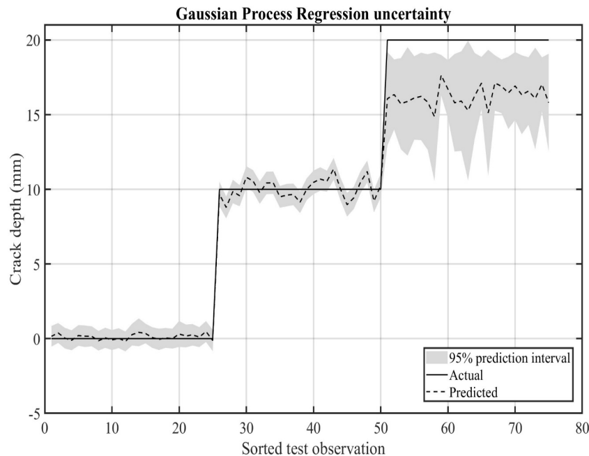
Figure 13. Prediction uncertainty of the Gaussian Process Regression
