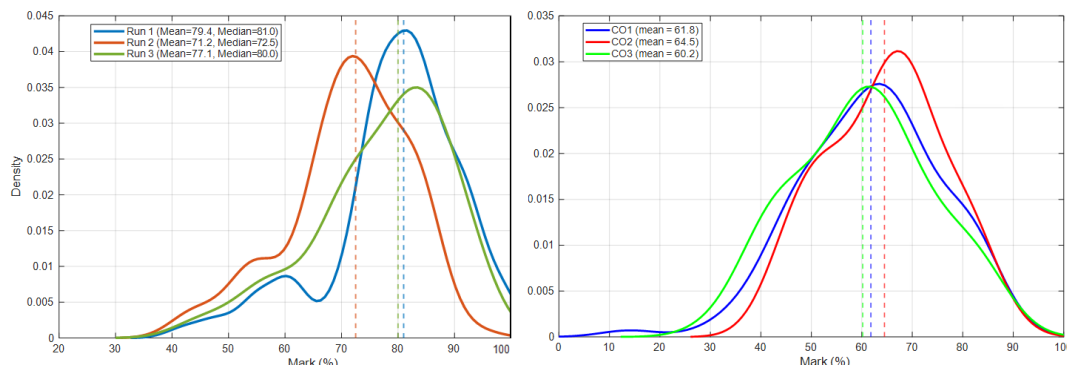
Figure 5. Distribution of marks generated across three repeated runs for both vision language models (VLMs): Gemini (left) and Copilot (right)
