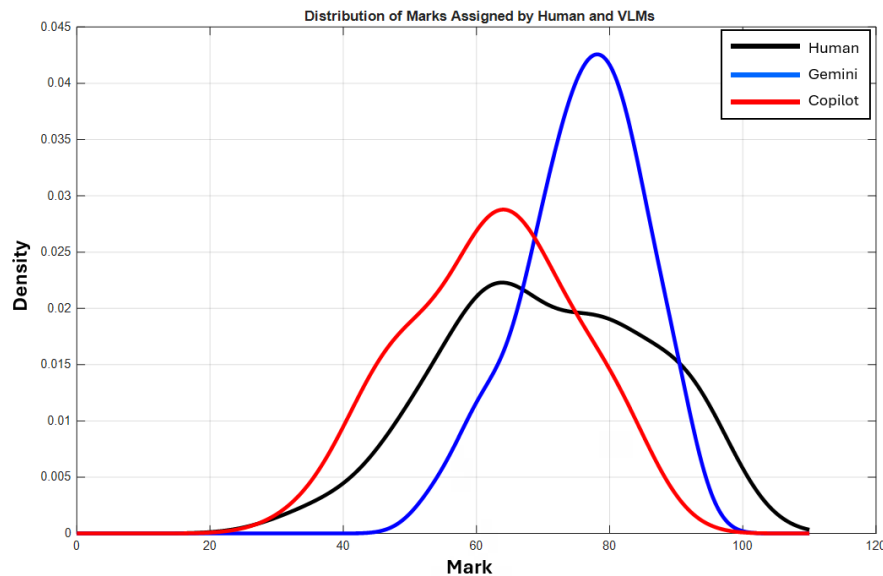
Figure 8. Density function plot showing marking trends for all assessors
