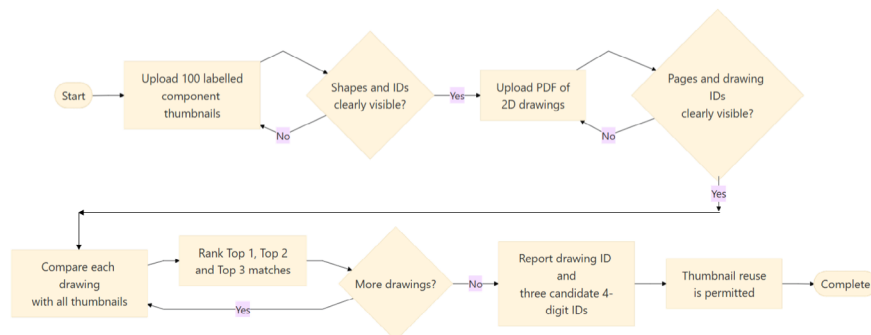
Figure 3. Flow chart of deployment for image sorting analysis
