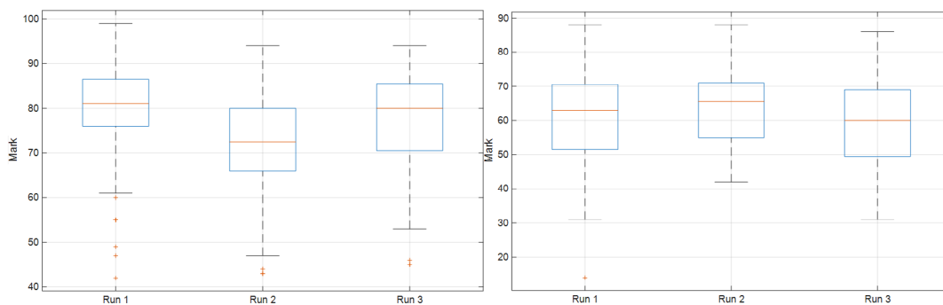
Figure 6. Boxplots show score distributions across three repeated grading runs for Gemini (left) and Copilot (right). Similar medians and interquartile ranges indicate broadly comparable scoring behavior across evaluations, although variability among individual drawings was observed.
