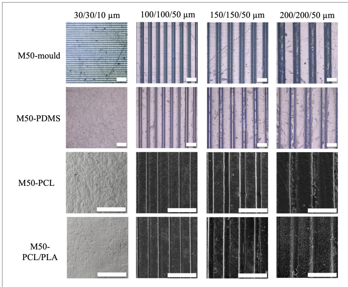
Figure S3. Light microscope images of M-50 3D-printed master mould and casted PDMS mould (scale bar: 200 μm) (top). SEM images of the PCL and PCL/PLA microgroove films casted from the PDMS mould (scale bar: 500 μm) (bottom).
