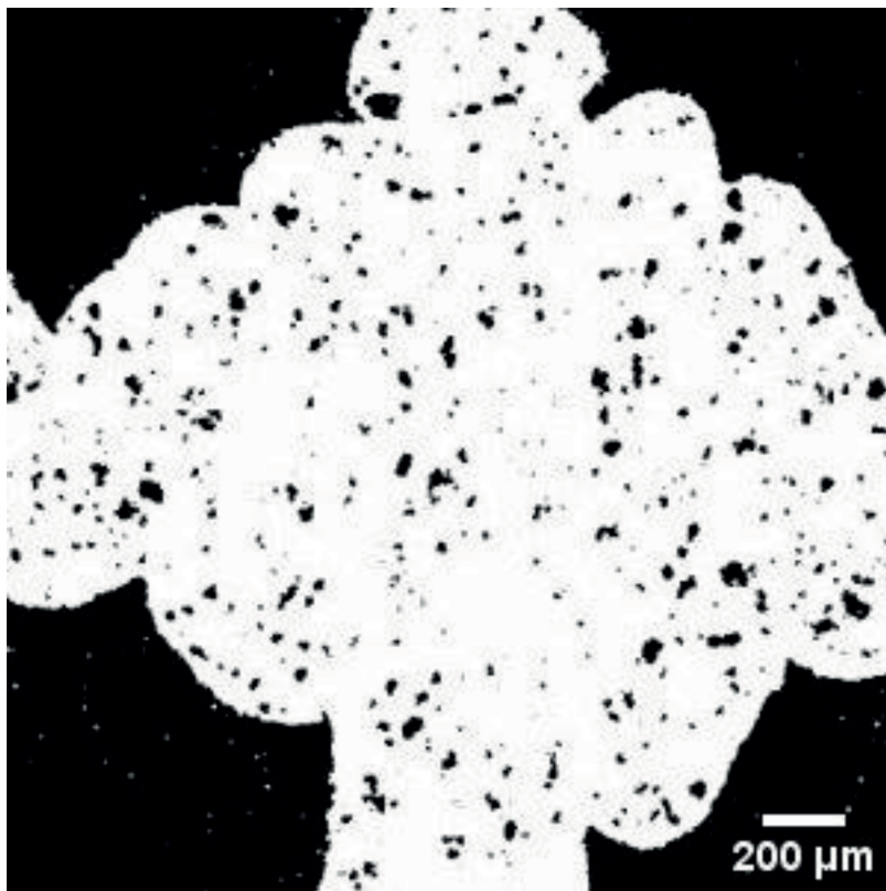
Figure S1. Image representing the microporosity ( <40 \mu\text{m} ) or closed porosity within the strands, extracted from the micro-computed tomography (CT) of the Schwarz structure.
