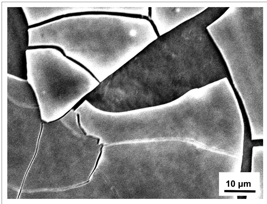
Figure S1. Surface morphology of the scaffold coated with 15 GS composite.
