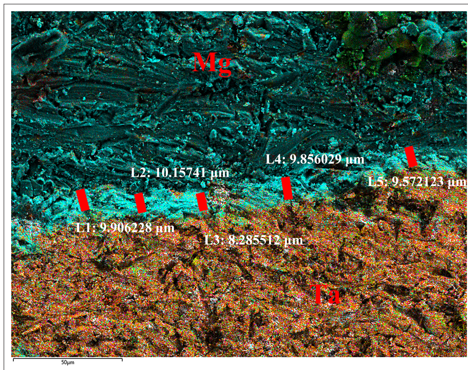
Figure S1. Thickness of the reaction layer in the Ta–Mg composite. Scale bar: 50 μm.
