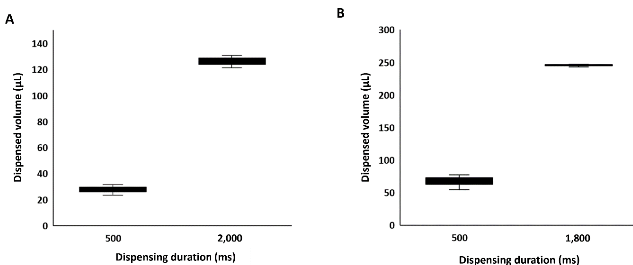
Figure S1. Volumetric dispensing modes. Repeatability comparison of volumetric dispensing modes (A) using a microfluidic device at valve opening times of 500 ms and 2,000 ms at 25 mbar, and (B) using a separate fluid line at valve opening times of 500 ms and 1,800 ms at 50 mbar.
