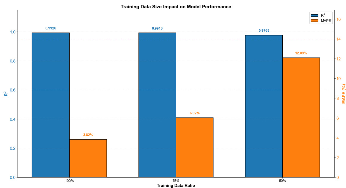
Figure S9. Comparative chart of different data quantities, showing that more than 315 well-distributed measurements are generally sufficient to achieve stable predictive performance Abbreviation: MAPE: Mean absolute percentage error.
