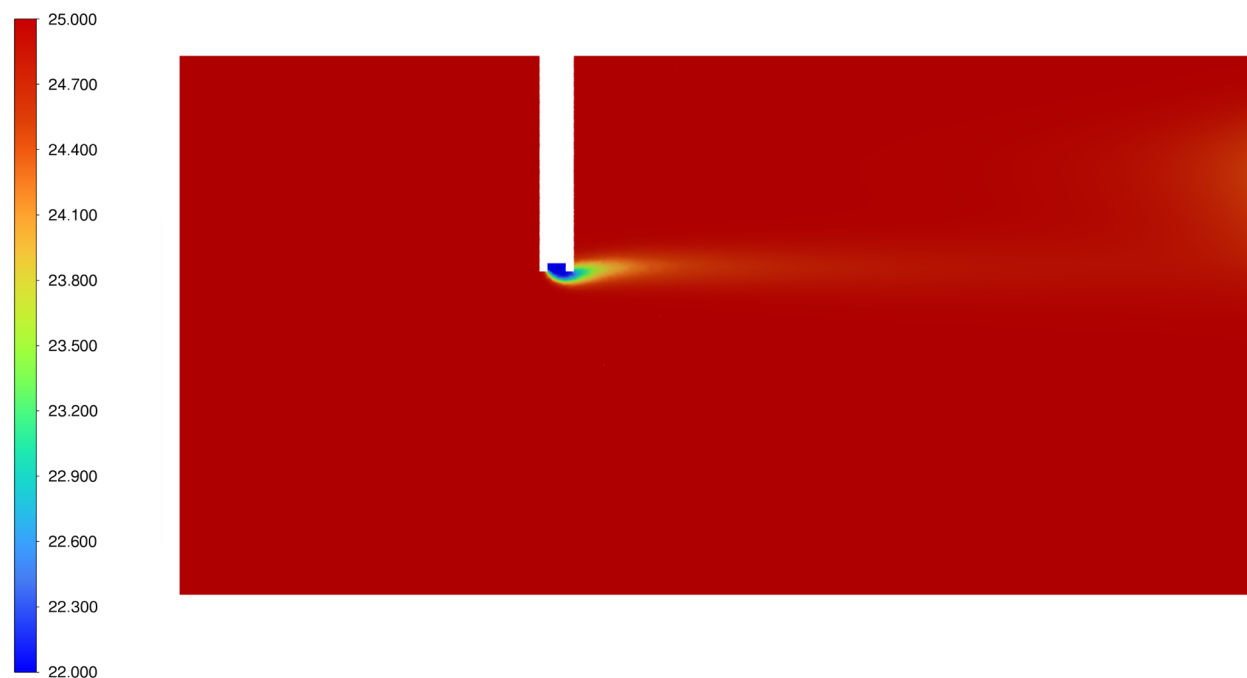
Figure S3. Temperature contour plot showing the transient heating process of the filament during deposition. The results indicate that the ink gradually warms up from 22 °C to the ambient supporting bath temperature of 25 °C over time.
