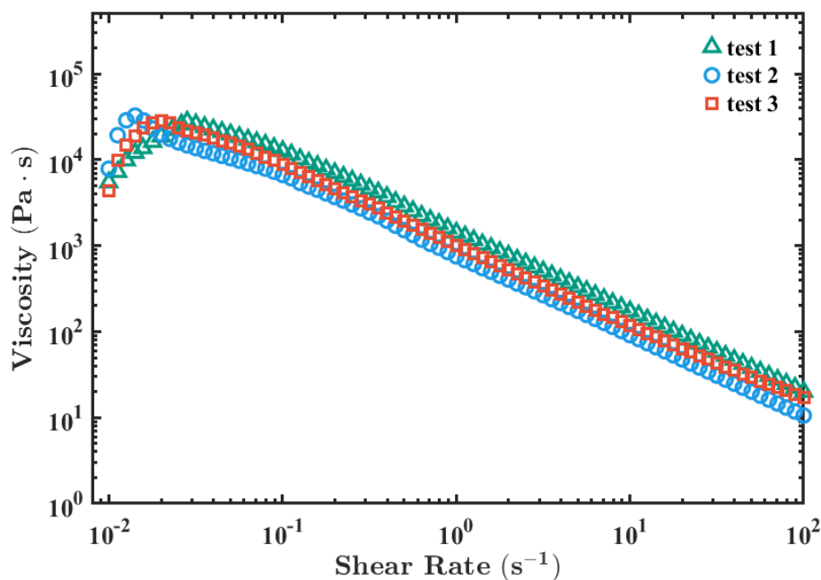
Figure S2. Repeatability assessment of rheological measurements at 25 °C. Three independent measurements were performed under identical experimental conditions. The resulting flow curves exhibited consistent trends and comparable rheological responses across replicates, demonstrating satisfactory measurement repeatability.
