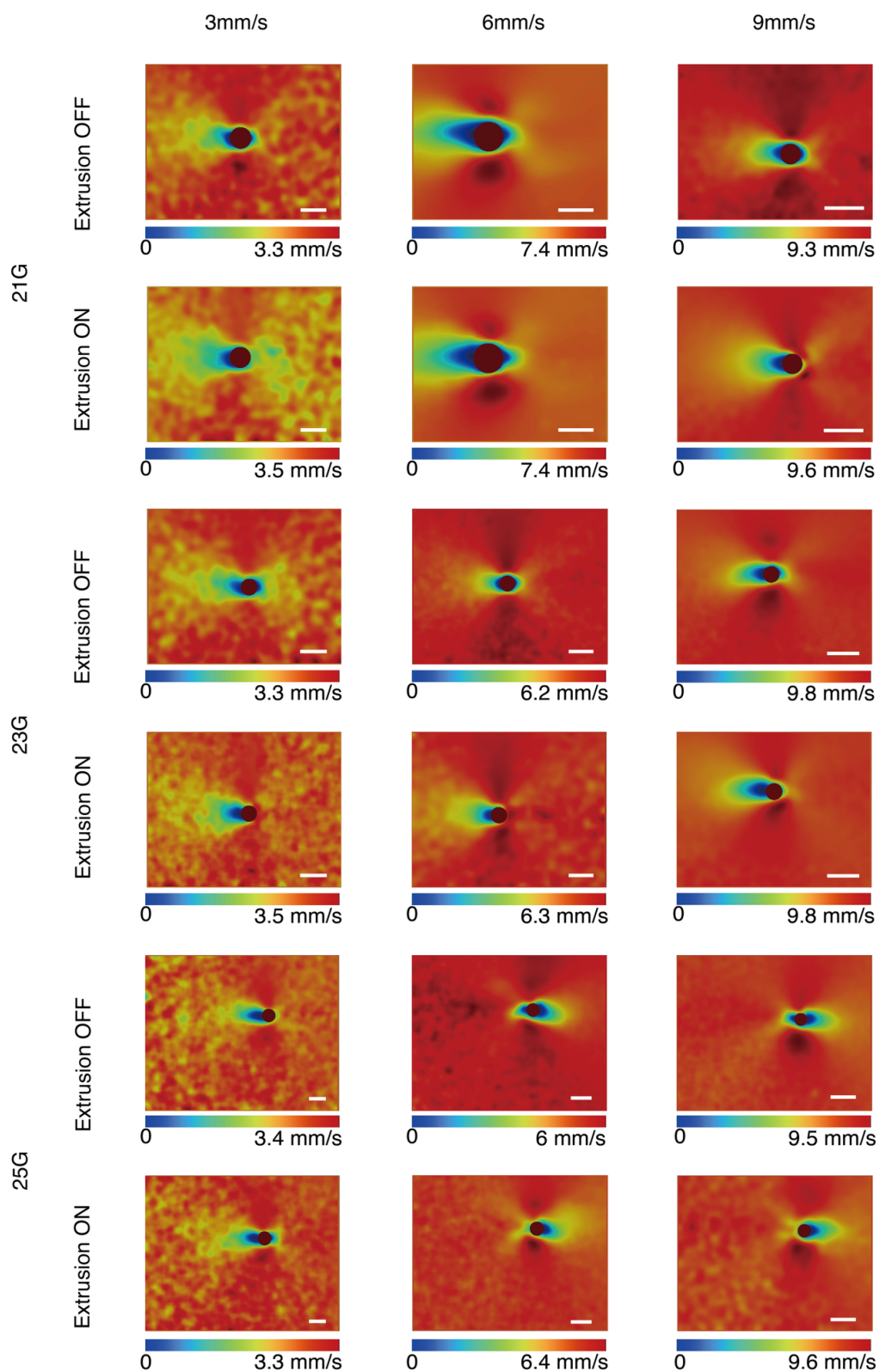
Figure S6. Influence of needle gauge and printing speed on the horizontal flow field (bottom view)
