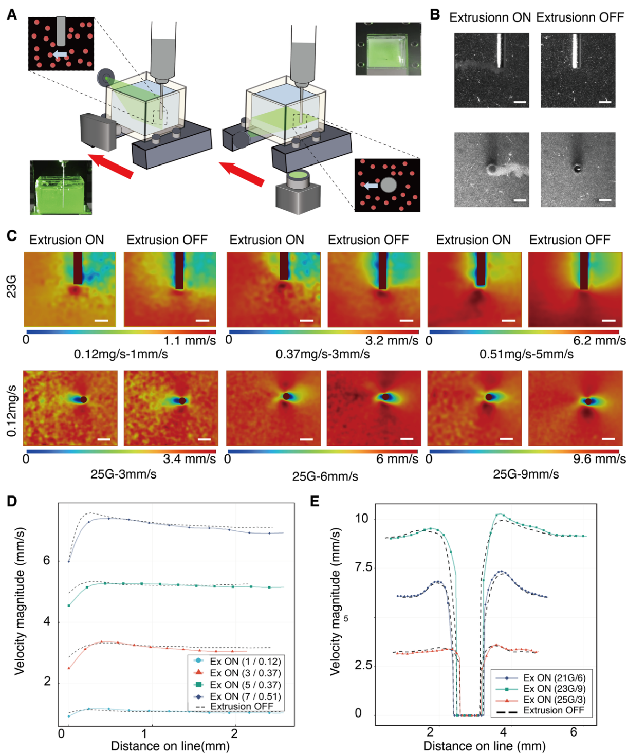
Figure S5. Particle image velocimetry (PIV) experimental setup and multi-dimensional flow field analysis. (A) Schematic illustration of the PIV system, including the laser-sheet orientation, camera positions for side and bottom views, and nozzle movement in the supporting bath. (B) Representative raw PIV images. (C) Velocity magnitude counter for various needle gauges and printing parameters. (D–E) Quantitative comparison of velocity magnitude profiles along specific lines in the side view (D) and bottom view (E).
