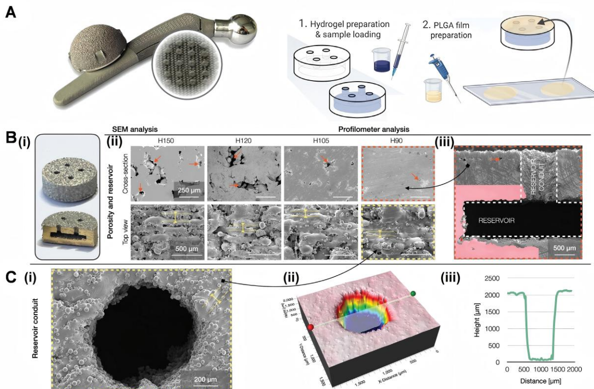
Figure 6. Structural integration strategy: (A) Real-scale implant and the preparation process of the hydrogel-dye loaded samples with a PLGA film; (B) Morphology and structural optimization of the 3D-printed samples: (i) macroscopic image and cross-section; (ii) trend of pore formation (red arrows) with decreasing hatching distance from 150 \mu\text{m} to 90 \mu\text{m} ; (iii) cross-sectional view of a sample printed with the final parameters, showing the integrated reservoir and delivery conduit; (C) Microstructural and topographical characterization of the reservoir and conduit (final parameters): (i, ii) images obtained by scanning electron microscopy (SEM) and optical profilometry, respectively; (iii) depth line profile of the reservoir measured by the profilometer. Reprinted with permission from 129 , Copyright (2024), John Wiley & Sons.
