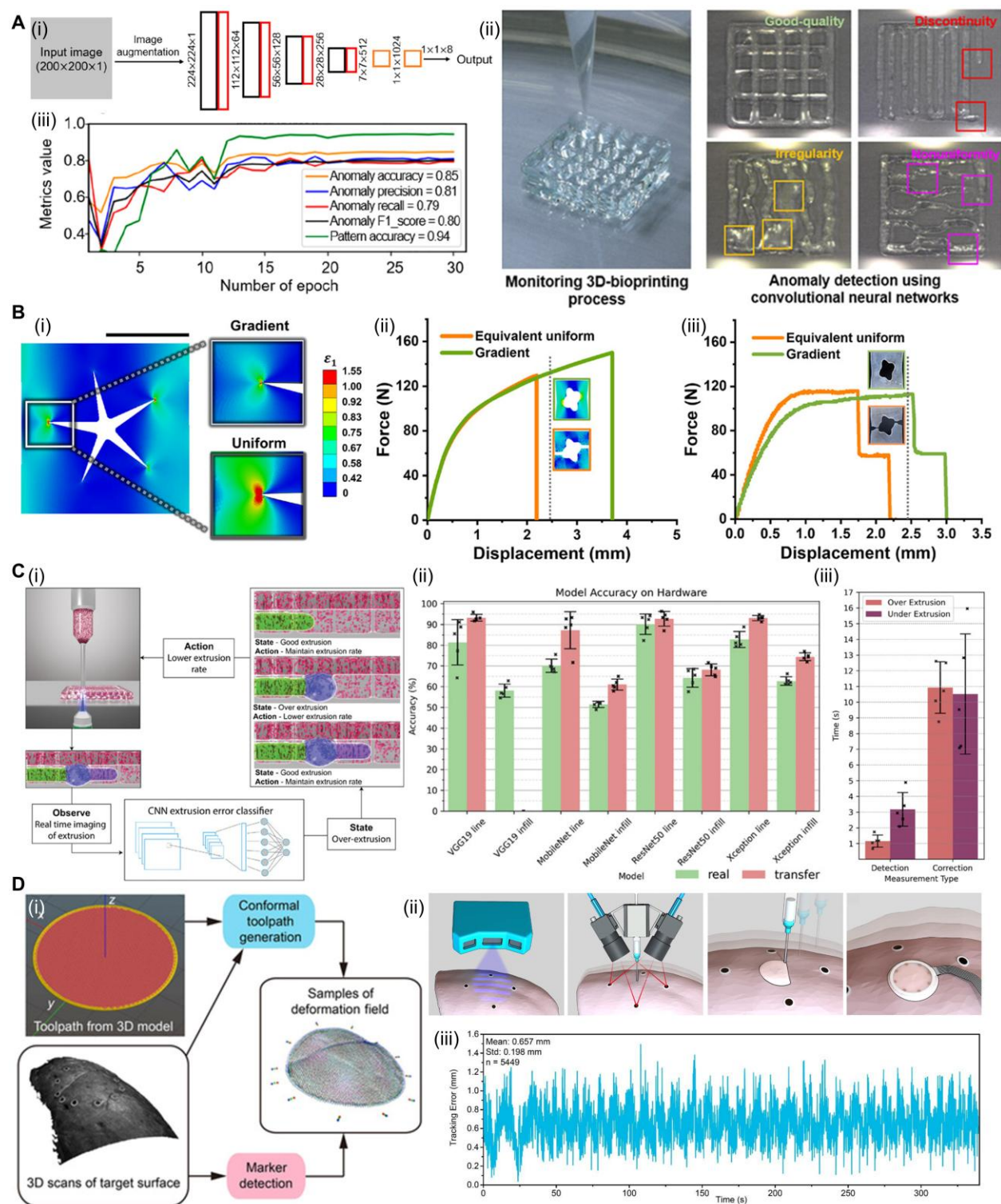
Figure 6. AI-assisted open-loop monitoring and closed-loop control in additive manufacturing. (A) CNN-based anomaly detection in extrusion bioprinting. (i) Open-loop flow diagram of the CNN model and model performance within 30 training epochs evaluated on the validation dataset. (ii). 3D-bioprinting process with anomaly detection using CNN. Reprinted with permission from Jin et al. 78 Copyright © 2023 ACS Publishing. (B) AI-guided grayscale DLP printing for programmable mechanical response. (i) Finite element strain distributions of structures printed with
