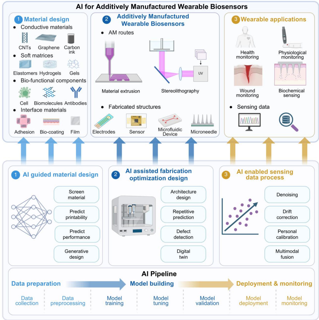
Figure 3. Three-stage AI workflow linking pre-printing design, in-process control, and post-printing applications in additively manufactured wearable biosensors.
