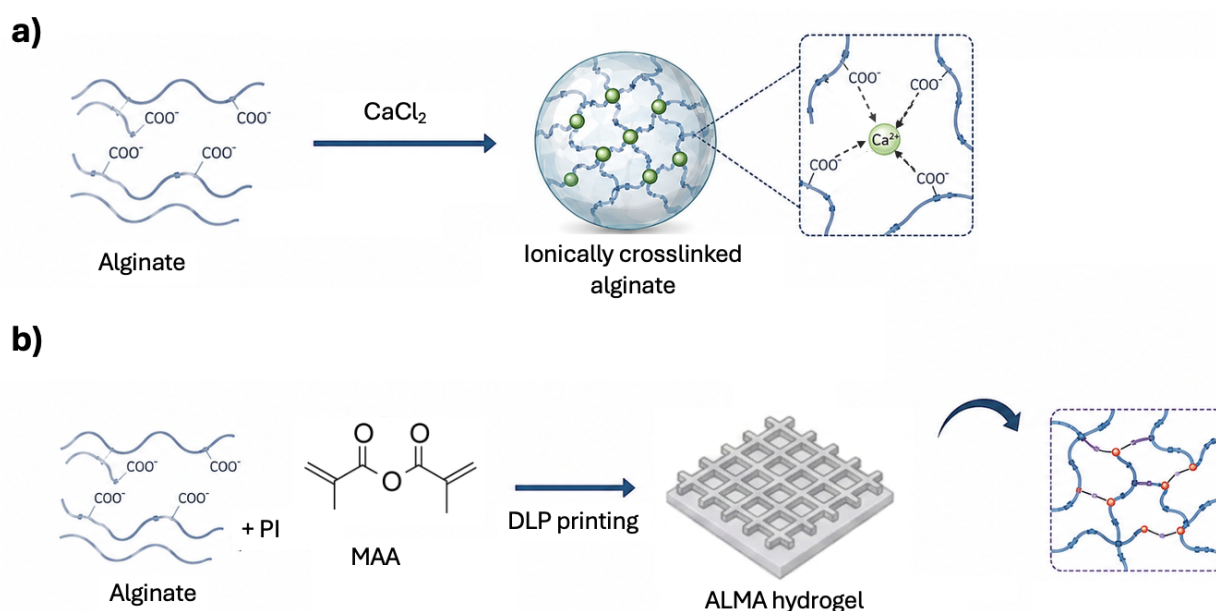
Figure 4. Ionic and covalent strategies for alginate hydrogels. (a) Ionically crosslinked alginate microbeads, and (b) 3D ALMA hydrogel fabrication using a 3D DLP printer.
