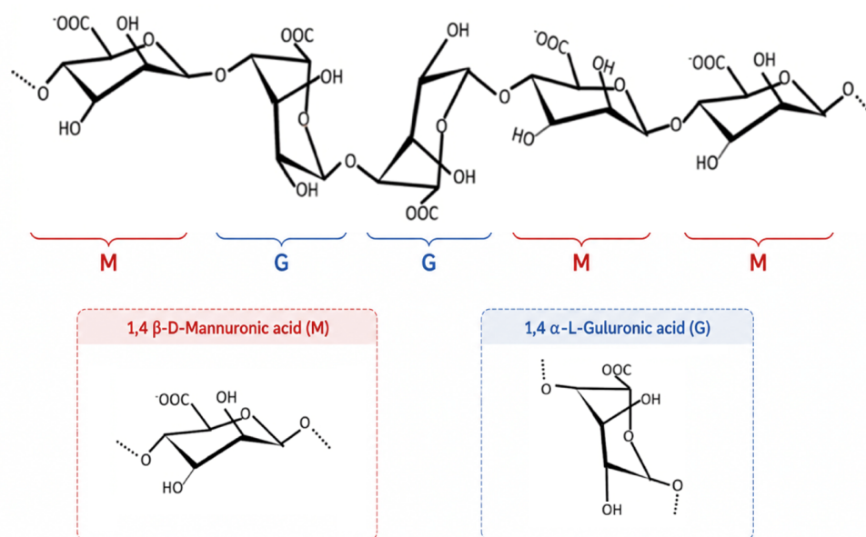
Figure 3. The chemical structure of alginate. Schematic created by the authors using PowerPoint and Gemini
