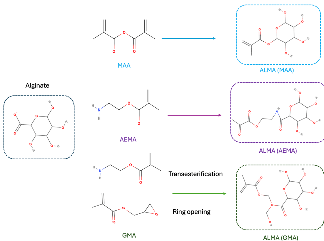
Figure 6. ALMA synthesis using MAA, AEMA, and GMA
