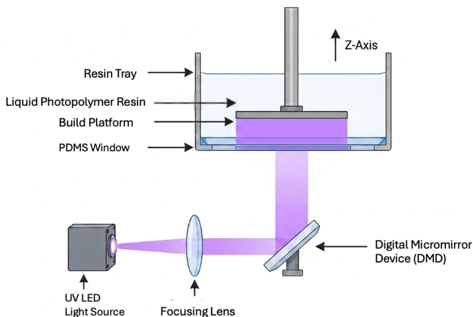
Figure 7. Working principle of DLP 3D printer
