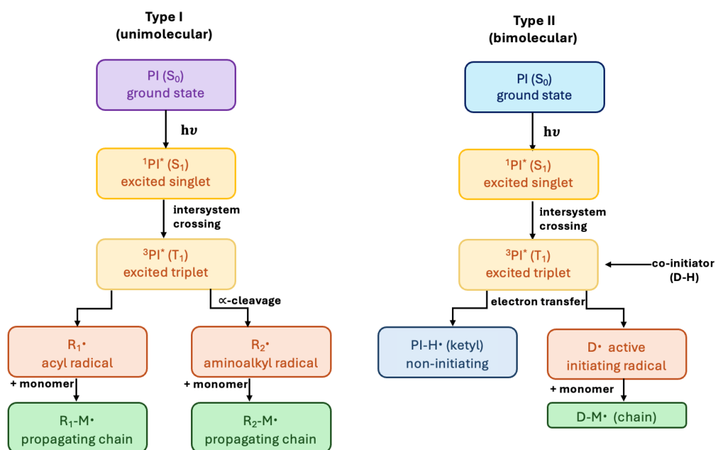
Figure 8. General reaction mechanisms of type I and type II photoinitiators. Type I initiators undergo direct \alpha -cleavage from the excited triplet state ( T_1 ) to generate two reactive radicals ( R_1\cdot and R_2\cdot ). Type II initiators require a co-initiator (D-H), and the T_1 state abstracts a hydrogen atom or undergoes electron transfer to yield a non-initiating ketyl radical (PI-H \cdot ) and an active initiating radical (D \cdot ).
