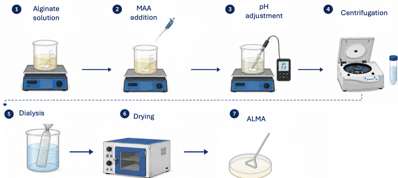
Figure 5. ALMA synthesis steps with MAA
