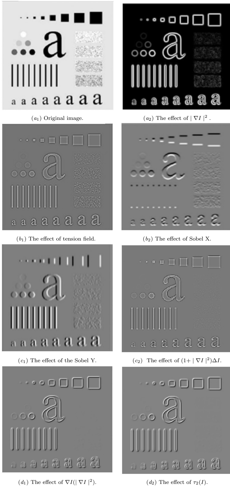
Figure 2. Evaluating the strengths and limitations of tension field versus 2-tension field in edge detection and noise suppression.
