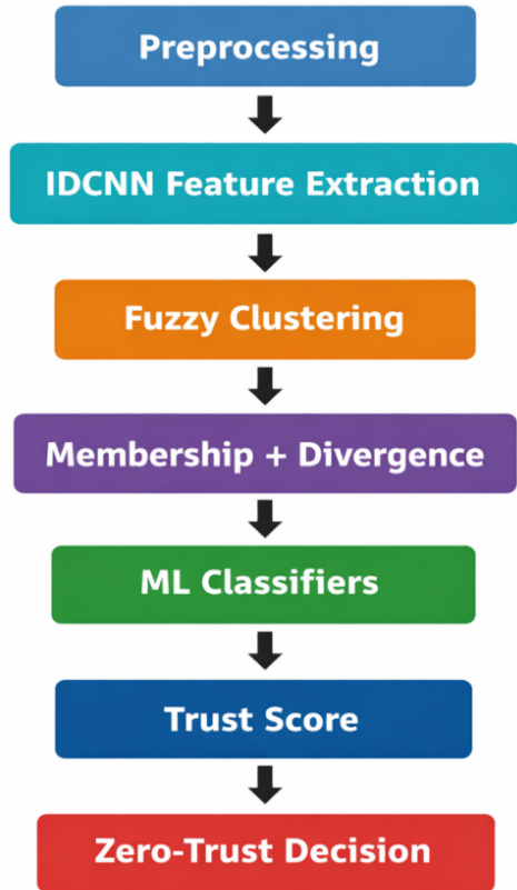
Figure 12. Zero-Trust decision model of data analysis. The input data were first preprocessed to clean and prepare them for analysis. An improved deep convolutional neural network (IDCNN) then extracted significant features; finally, fuzzy clustering and membership-divergence analysis determined the data's similarities and uncertainties. Lastly, machine learning (ML) classifiers calculated a trust score to inform the ultimate Zero-Trust security decision.
