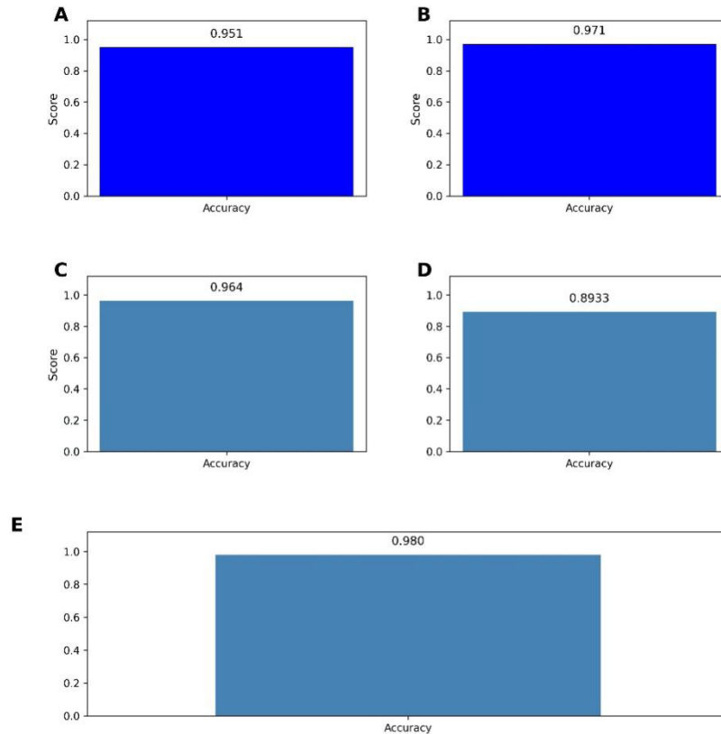
Figure 6. Accuracy comparison of multiple machine learning models. (A) Decision tree. (B) Logistic regression. (C) Random forest. (D) K-nearest neighbors (KNN). (E) Support vector machine (SVM).
