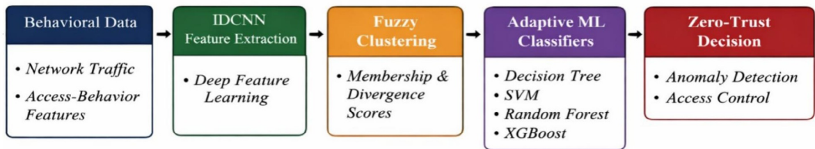
Figure 1. Hybrid intrusion detection system flowchart
