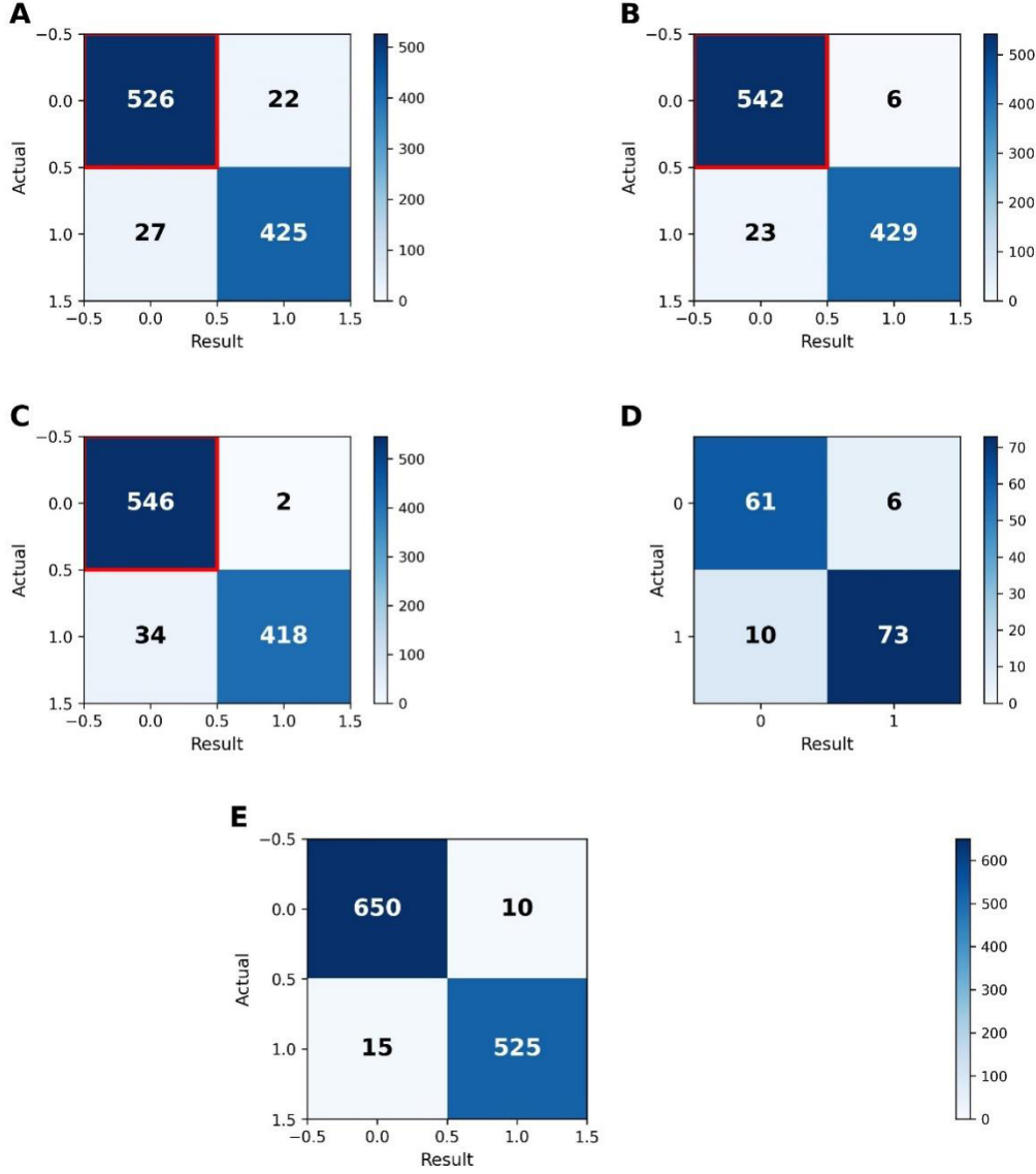
Figure 9. The image compares confusion matrices for decision tree, logistic regression, random forest, K-nearest neighbors (KNN), and support vector machine (SVM) models, showing prediction accuracy and misclassification counts. The SVM model achieves the highest accuracy with the fewest false predictions. (A) Decision tree. (B) Logistic regression. (C) Random forest. (D) K-nearest neighbors (KNN). (E) SVM.
