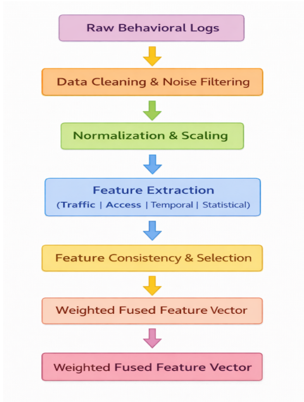
Figure 3. Data preprocessing and feature engineering pipeline
