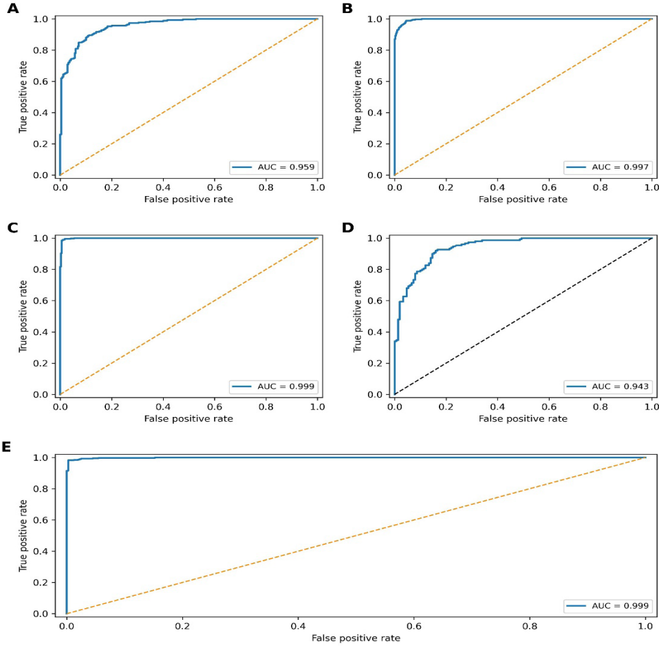
Figure 10. Receiver operating characteristic (ROC) curves for the evaluated classification models: (A) decision tree, (B) logistic regression, (C) random forest, (D) K-nearest neighbors (KNN), and (E) support vector machine (SVM). Random forest and SVM achieved the highest area under the curve (AUC) of 0.999, indicating excellent discriminative performance.
