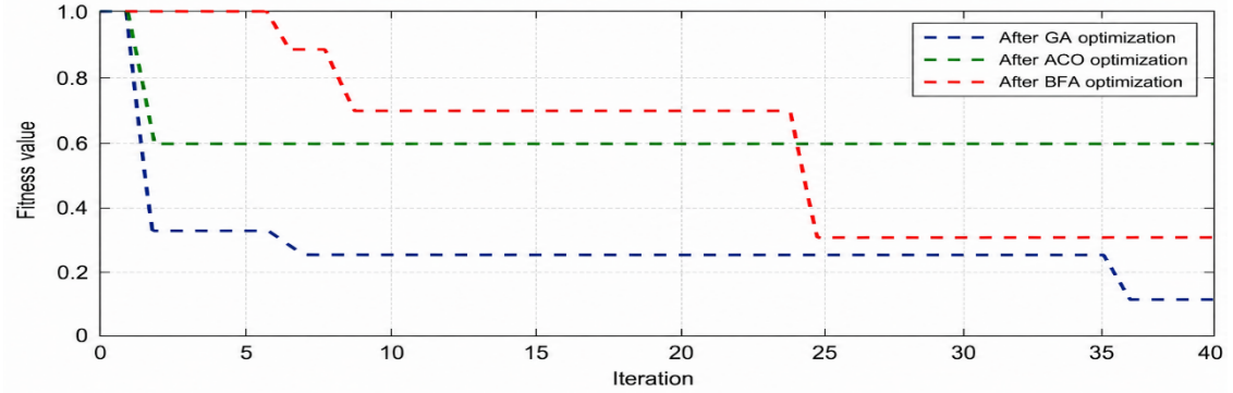
Figure 17. Convergence plot for 69- bus system
