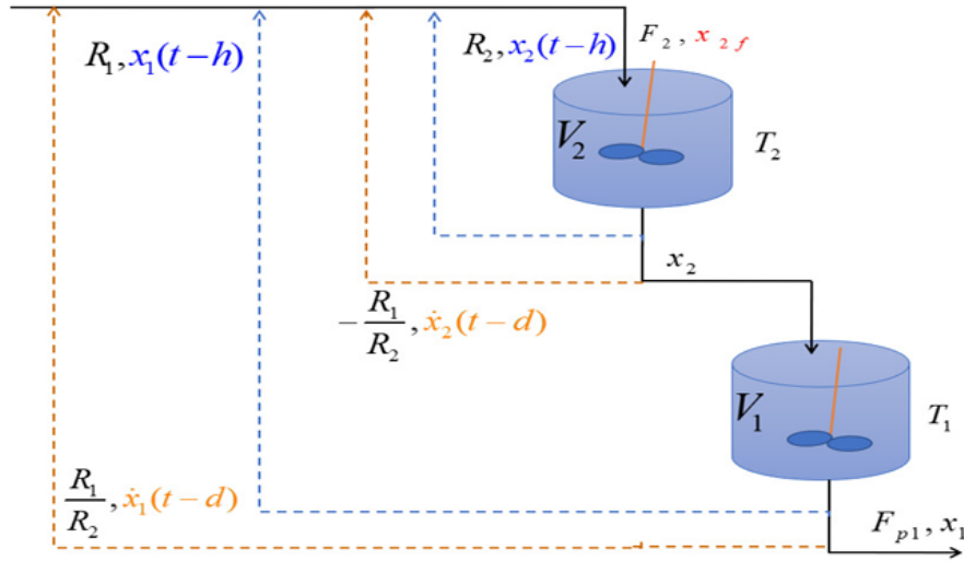
Figure 3. Two-stage chemical reactor with neutral time delay
