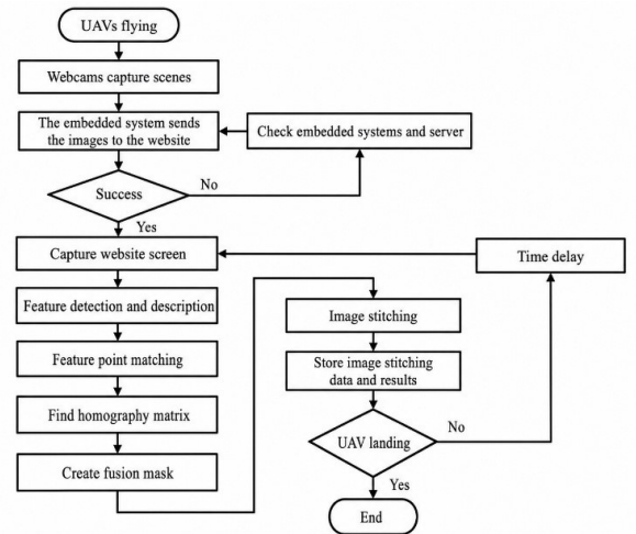
Figure 24. The real-time image-stitching process
