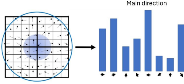
Figure 8. Histogram of main directions of keypoints
