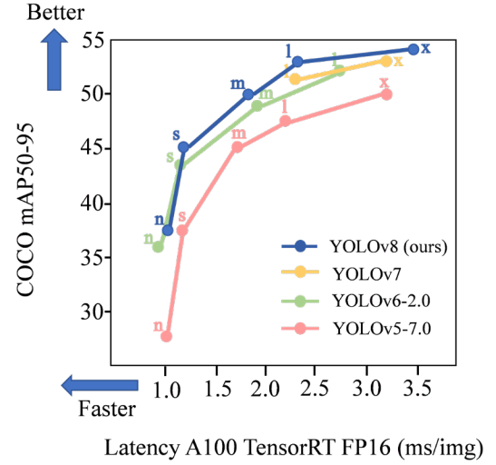
Figure 20. Comparison of various object detectors
