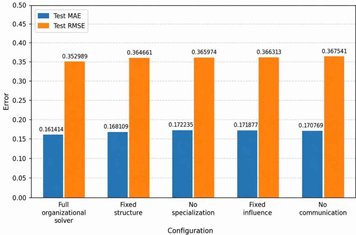
Figure 7. Comparative error performance of baseline and organizational models Abbreviations: MAE: Mean absolute error; RMSE: Root mean-squared error.
