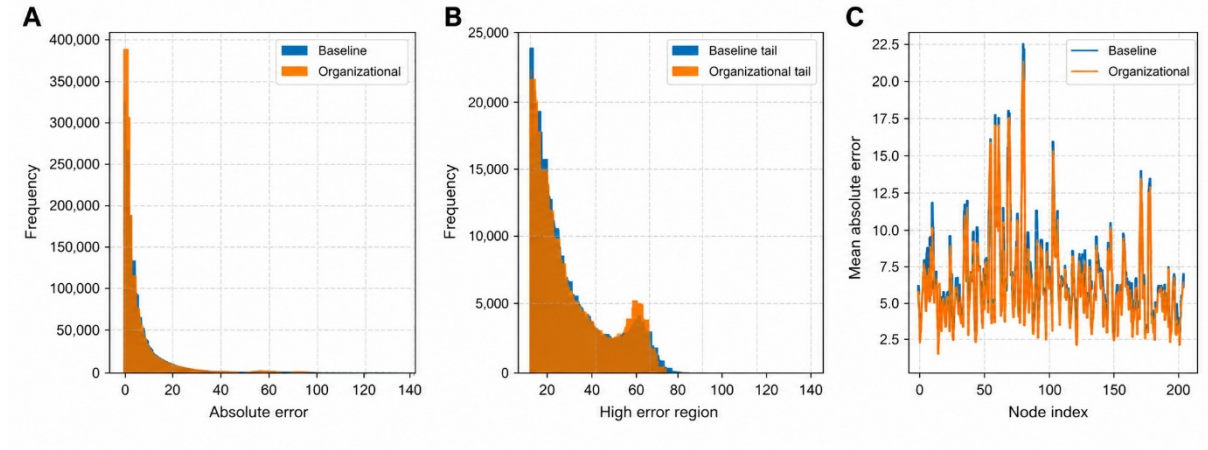
Figure 9. Advanced error analysis of baseline and organizational models. (A) Full error distribution. (B) Tail error analysis. (C) Per-node error density.
