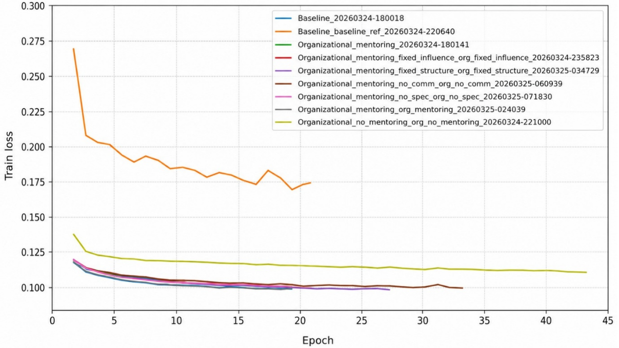
Figure 5. Training loss curves of the baseline and organizational traffic estimation models during training
