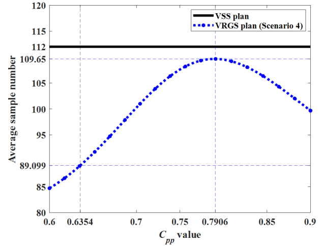
Figure 8. The average sample number curve of the C_{pp} -VSS and C_{pp} -VRGS plans
