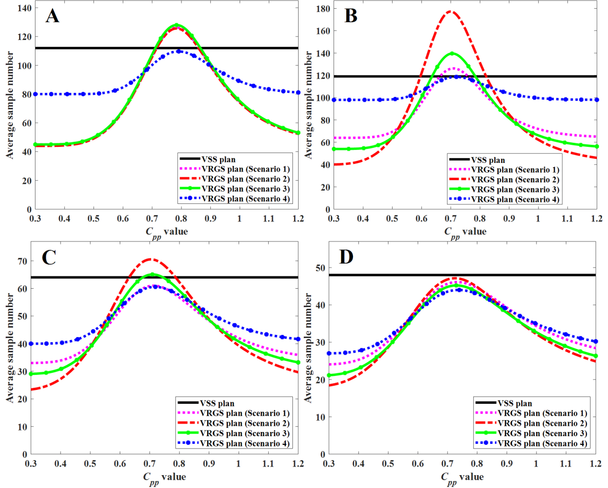
Figure 2. Average sample number curves of the C_{pp} -VSS and C_{pp} -VRGS plans with four scenarios under (b_{AQL}, b_{RQL}) = (0.5917, 1.000) and different risk levels. (A) (\alpha, \beta) = (0.01, 0.05) . (B) (\alpha, \beta) = (0.05, 0.01) . (C) (\alpha, \beta) = (0.10, 0.05) . (D) (\alpha, \beta) = (0.10, 0.10) .
