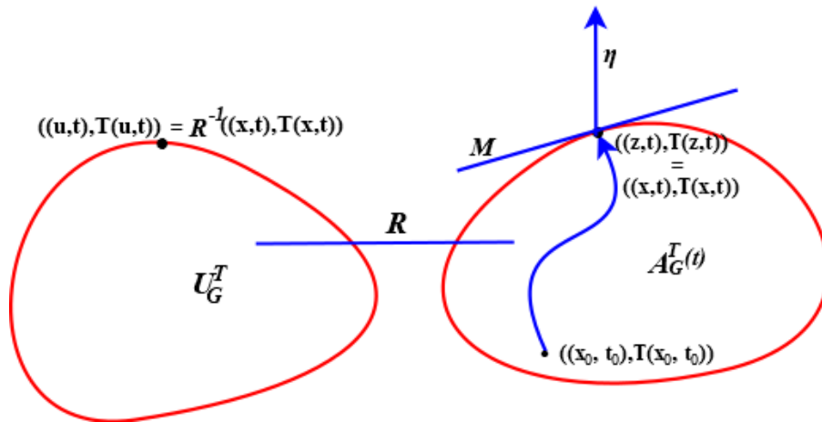
Figure 1. Geometric illustration of the exposed point property of the attainable set A_G^T(t) \subseteq X . The terminal point ((z, t), T(z, t)) is an exposed point of A_G^T(t) determined by the supporting hyperplane M and its outward normal vector \eta and is associated with the corresponding unique time optimal control ((u, t), T(u, t))^* \in U_G^T in the Frechet graph space G_T for the normal system at the minimum time t = t_1 , where ((u, t), T(u, t))^* = \text{sgn}[\eta' Y(t)] with \eta' denoting the transpose of vector \eta , and Y(t) = X^{-1}B(t) is the output space. In contrast, for the proper system, the time-optimal control need not be unique.
