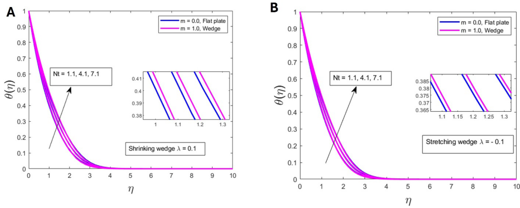
Figure 7. Temperature profiles \theta for different values of Nt on (A) shrinking wedge and (B) stretching wedge. Parameters: \lambda_T = 0.1; \lambda_C = 0.1; Pr = 7.0; Sc = 1.1; W = 7.1; Q = 6.1; Rd = 10.1; Nb = 10.0; \gamma = \frac{\pi}{6}; M = 5.0 .
