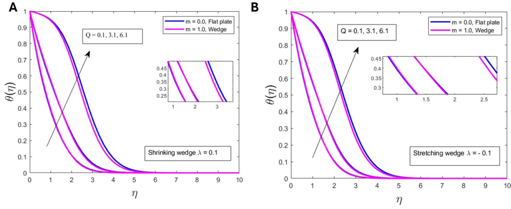
Figure 5. Temperature profiles \theta for different values of Q on (A) shrinking wedge and (B) stretching wedge. Parameters: \lambda_T = 0.1; \lambda_C = 0.1; Pr = 7.0; Sc = 1.1; W = 7.1; Rd = 10.1; Nt = 0.1; Nb = 10.0; \gamma = \frac{\pi}{6}; M = 5.0 .
