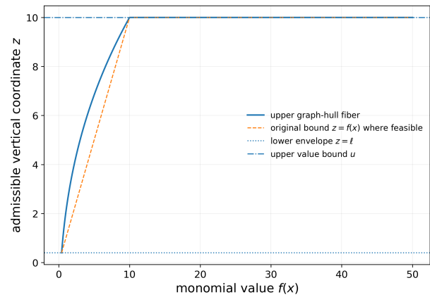
Figure 5. Vertical fiber of the graph hull for a \beta > 1 instance as a function of the monomial value f(x) . The lower endpoint is z = \ell , and the upper endpoint is the minimum of u and the secant-conic upper envelope.
