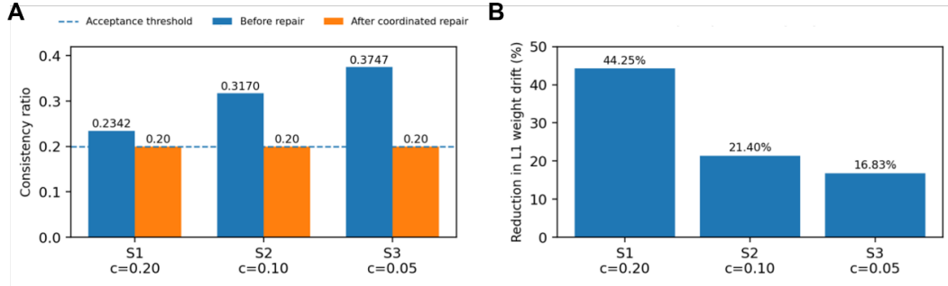
Figure 4. Visual summary of the independent inconsistency stress test. (A) Consistency recovery. (B) Disturbance reduction.
