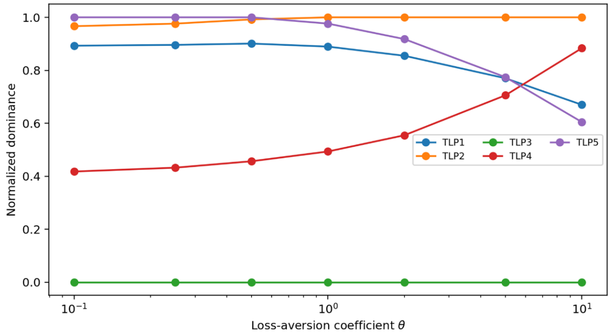
Figure 6. Sensitivity of normalized dominance values to the TODIM loss parameter
