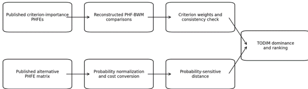
Figure 2. Data-processing procedure of the empirical case
