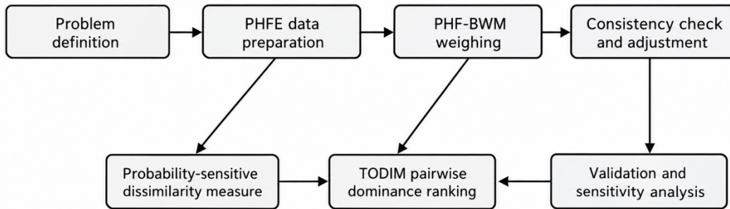
Figure 1. Research framework of the proposed PHF-BWM-TODIM method
