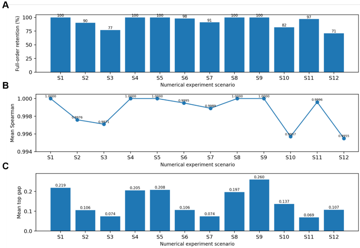
Figure 7. Visual summary of the scenario-based numerical experiments. (A) Ranking stability across data scales. (B) Spearman rank correlation across scenarios. (C) Average separation of the leading alternatives across scenarios.
