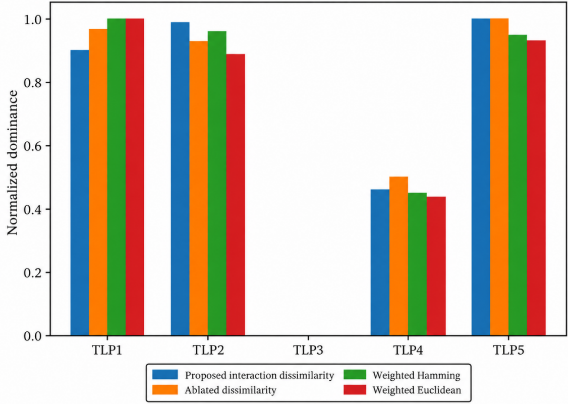
Figure 5. Alternative scores under four dissimilarity settings
