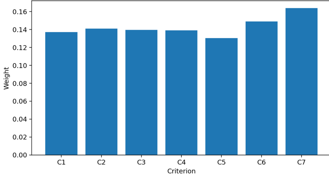
Figure 3. Criterion weights obtained by the reconstructed PHF-BWM
