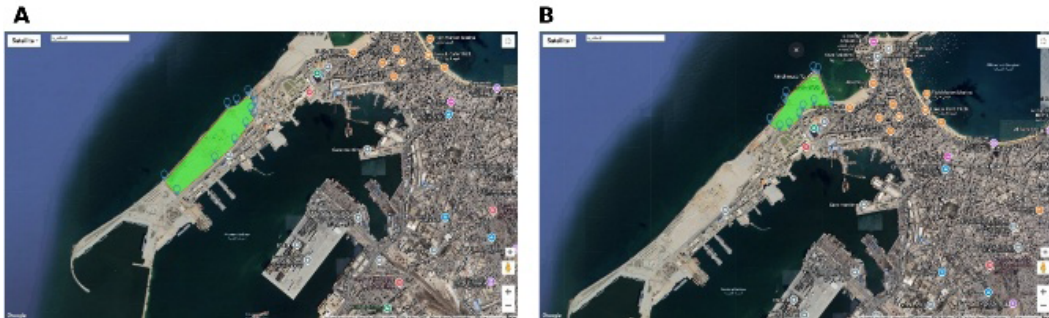
Figure 20. Identified onshore photovoltaic (PV) installation areas at Alexandria Port. (A) PV Area 1 assigned to the 1.5 MW PV array. (B) PV Area 2 assigned to the 0.5 MW PV array.
