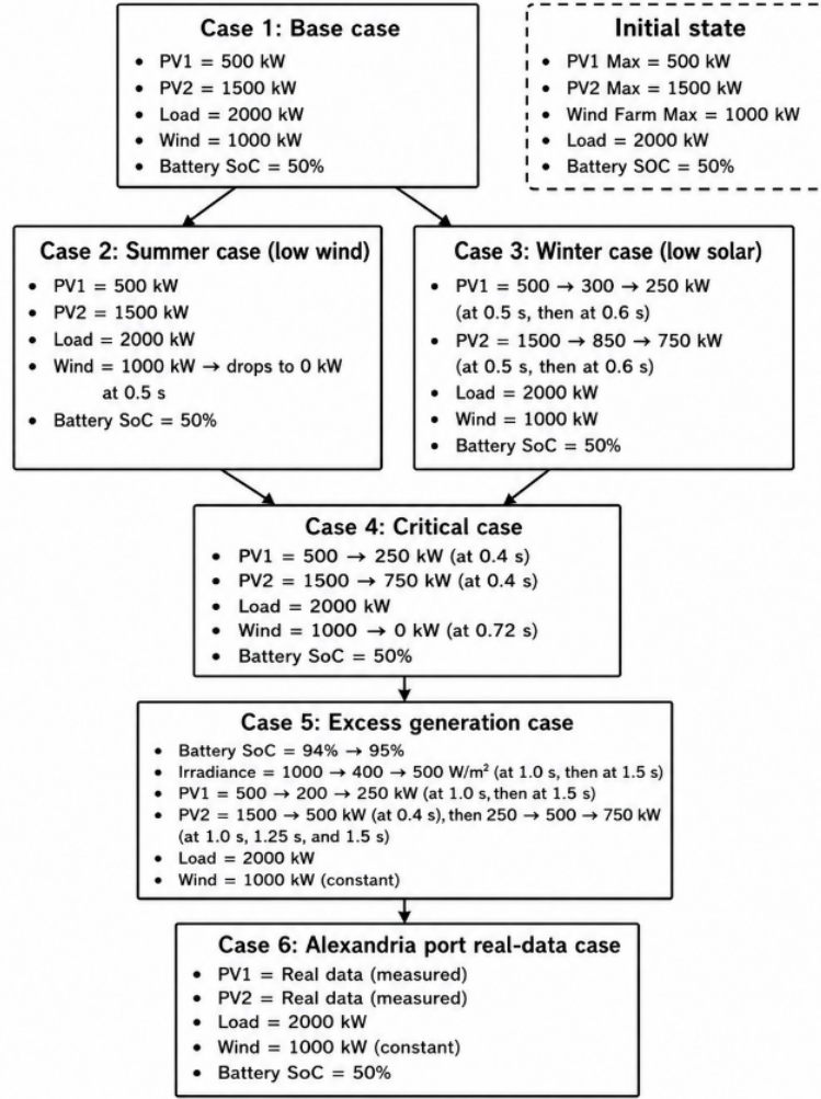
Figure 14. Simulation scenarios used to evaluate the conventional EMS under normal operation, renewable-power shortage, excess-generation, and real-data operating conditions
