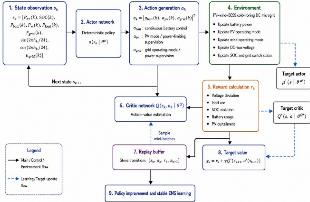
Figure 13. DDPG-based EMS workflow showing state observation, actor action generation, environment update, reward calculation, critic evaluation, replay-buffer learning, and target-network update
