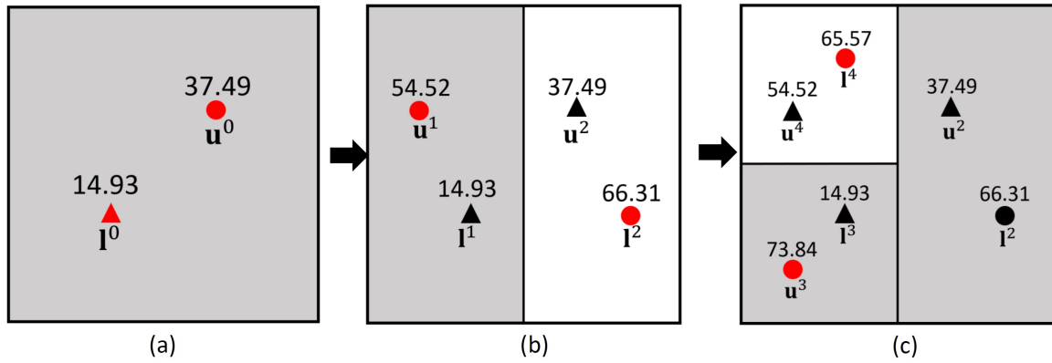
Figure 2. Sampling and partitioning rectangles using the BIRECT algorithm on the 2D Griewank function
