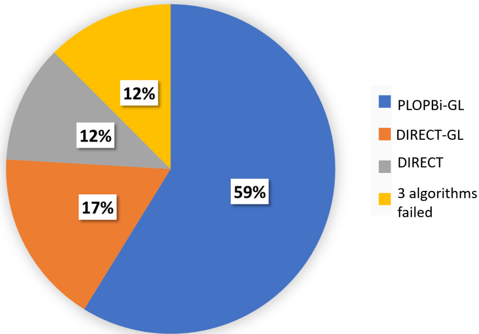
Figure 5. Performance of the PLOPBi-GL, DIRECT-GL, and DIRECT on the Hedar test functions with four pe
