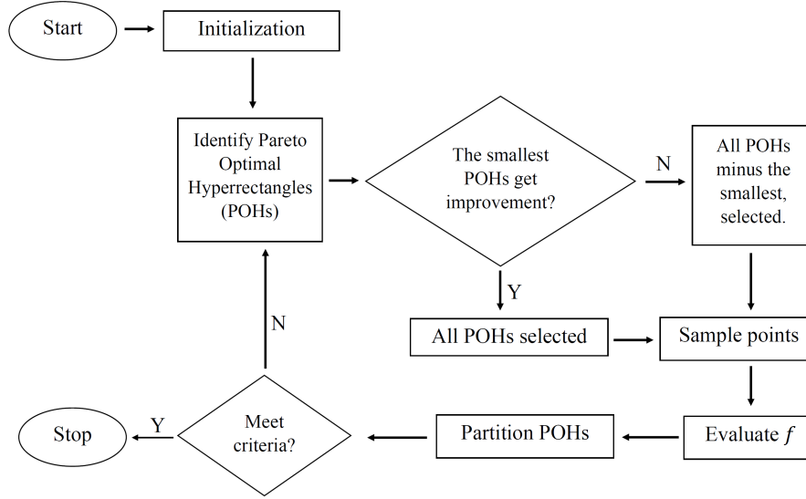
Figure 4. Flow chart of the PLOBi algorithm with parameter
