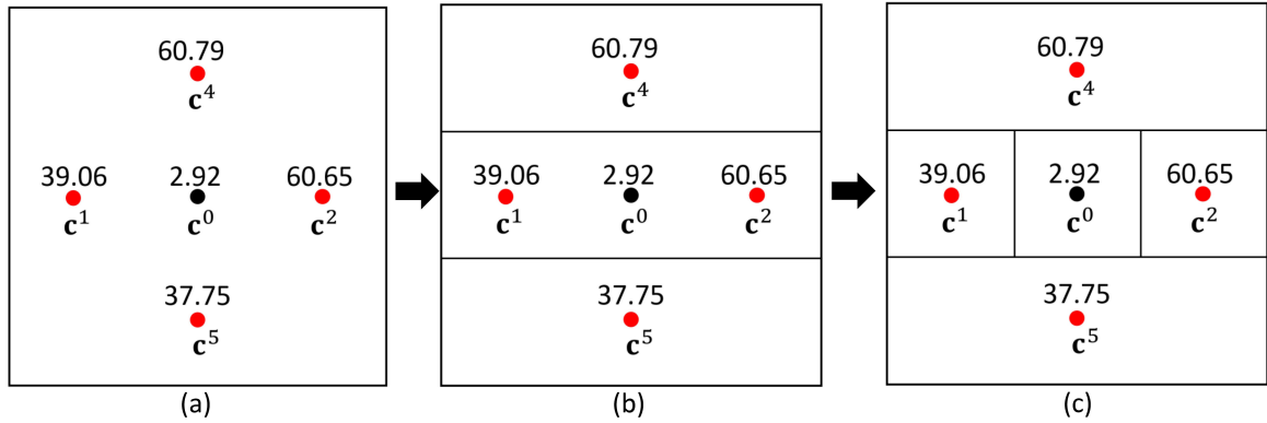
Figure 1. Sampling and partitioning rectangles using the DIRECT algorithm on the 2D Griewank function
