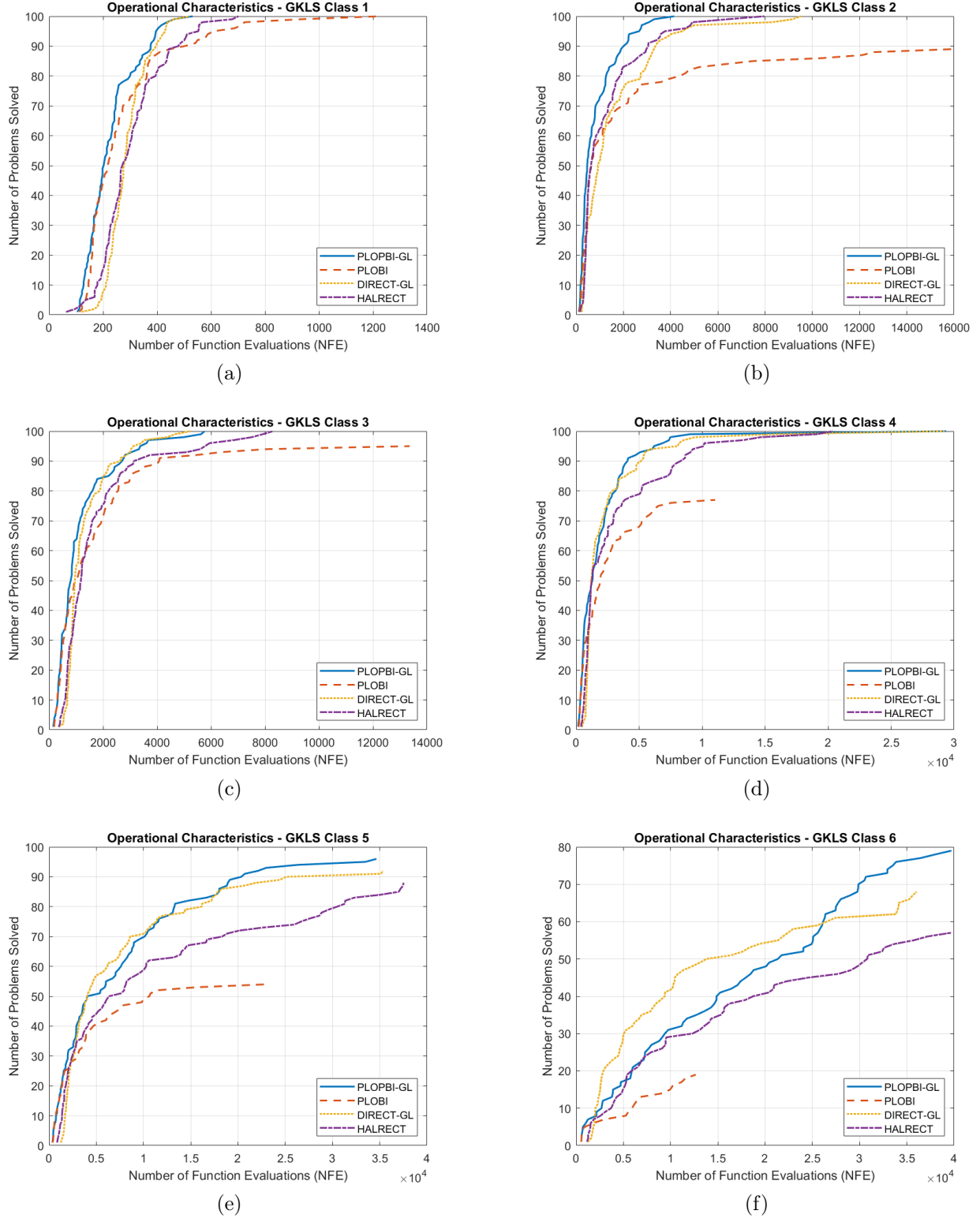
Figure 6. Number of successfully solved GKLS problems for dimensions n = 2, 3, 4
