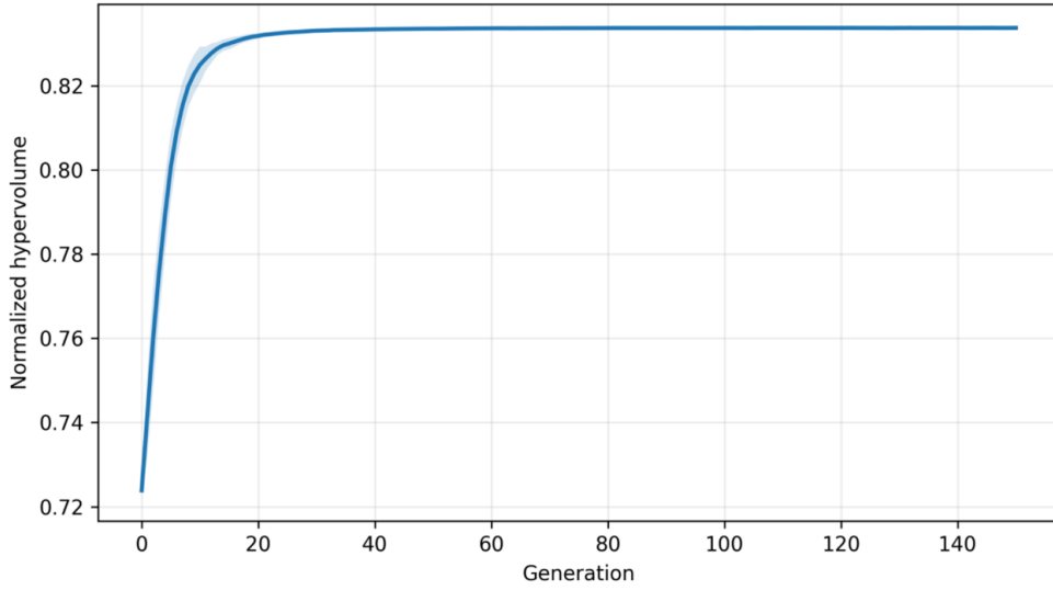
Figure 5. Mean normalized hypervolume across 30 independent non-dominated sorting genetic algorithm II runs; the shaded band represents \pm 1 standard deviation
