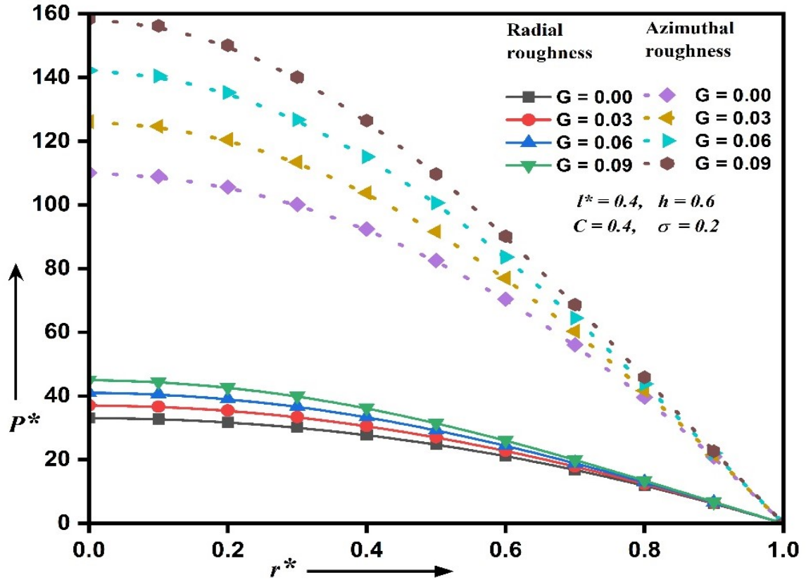
Figure 3. Graphical analysis of P^* versus r^* for a range of G values
