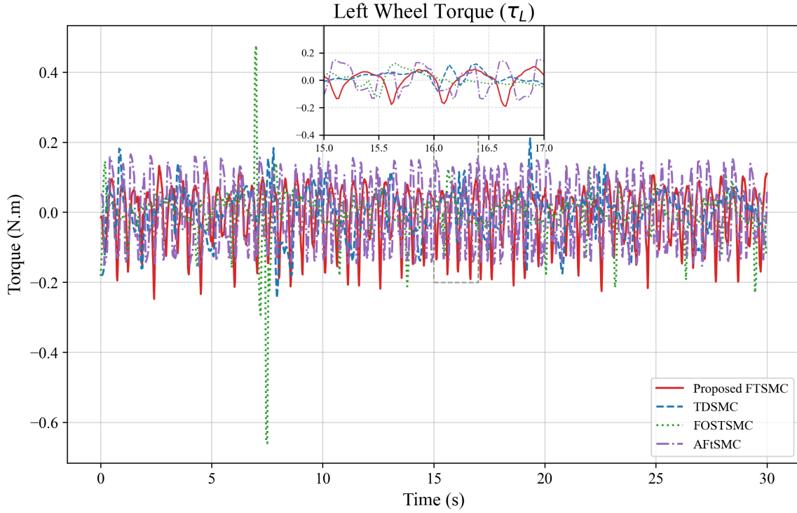
Figure 16. Control input: \tau_L with disturbance
