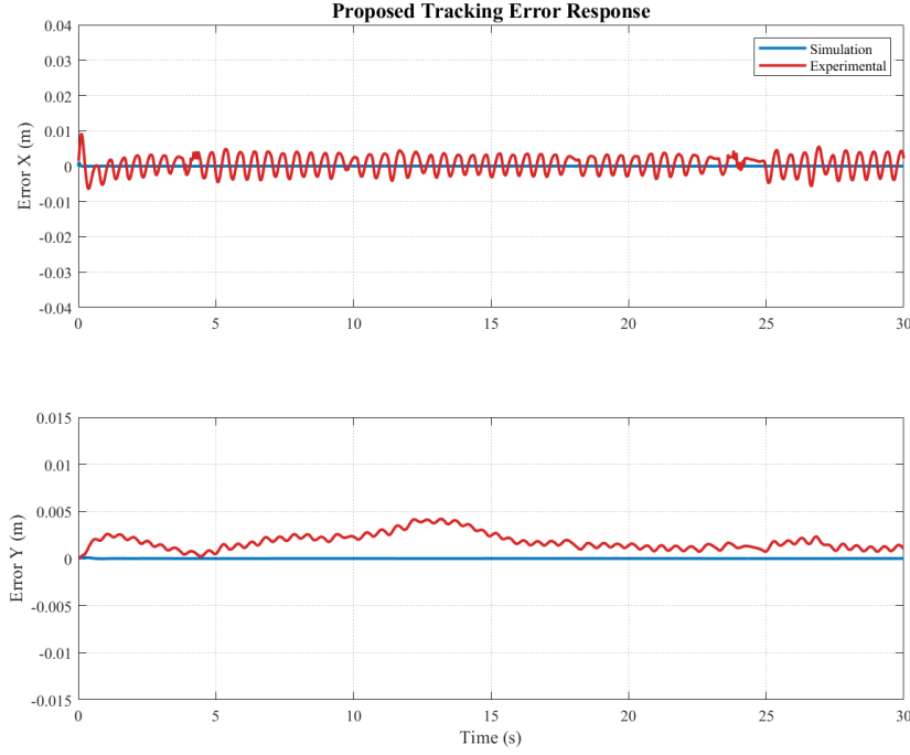
Figure 19. Proposed tracking error performance (simulation and experiment)
