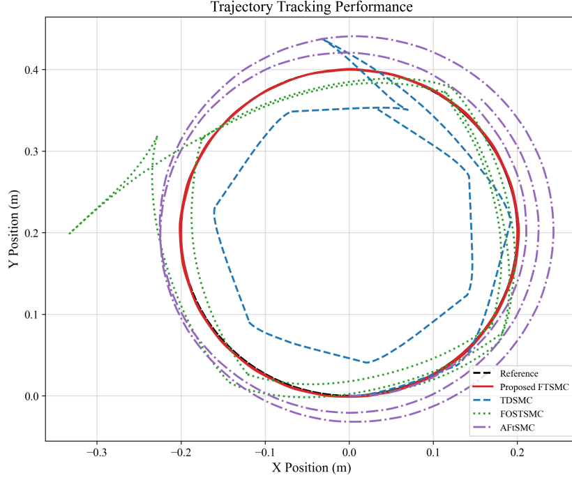
Figure 10. Comparison of trajectory tracking performance in the X-Y plane
