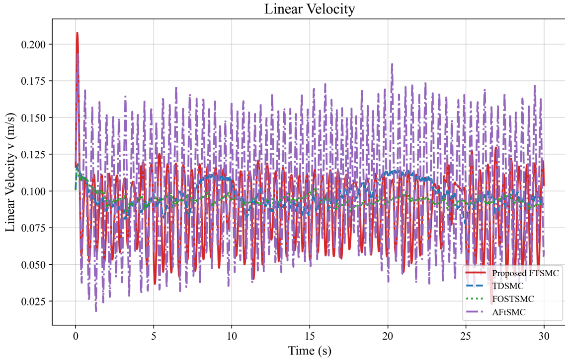
Figure 6. Linear velocity tracking ( v_c vs. v ) without disturbance
