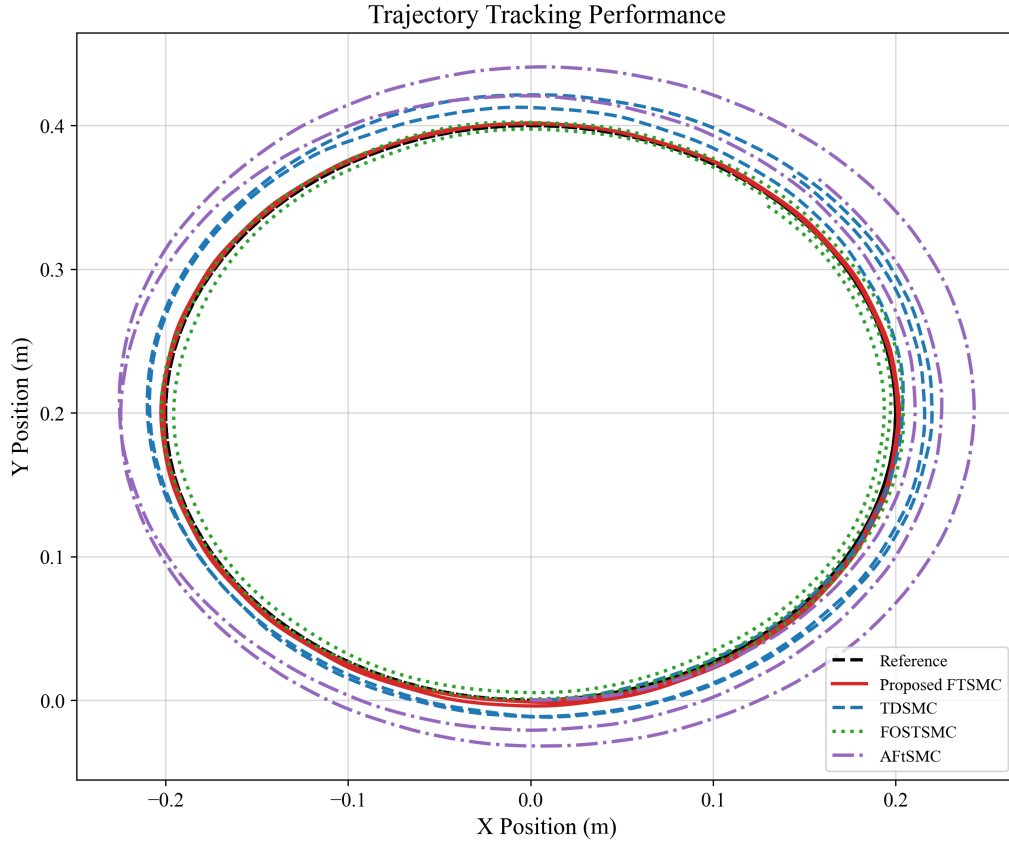
Figure 3. Comparison of trajectory tracking performance in the X-Y plane
