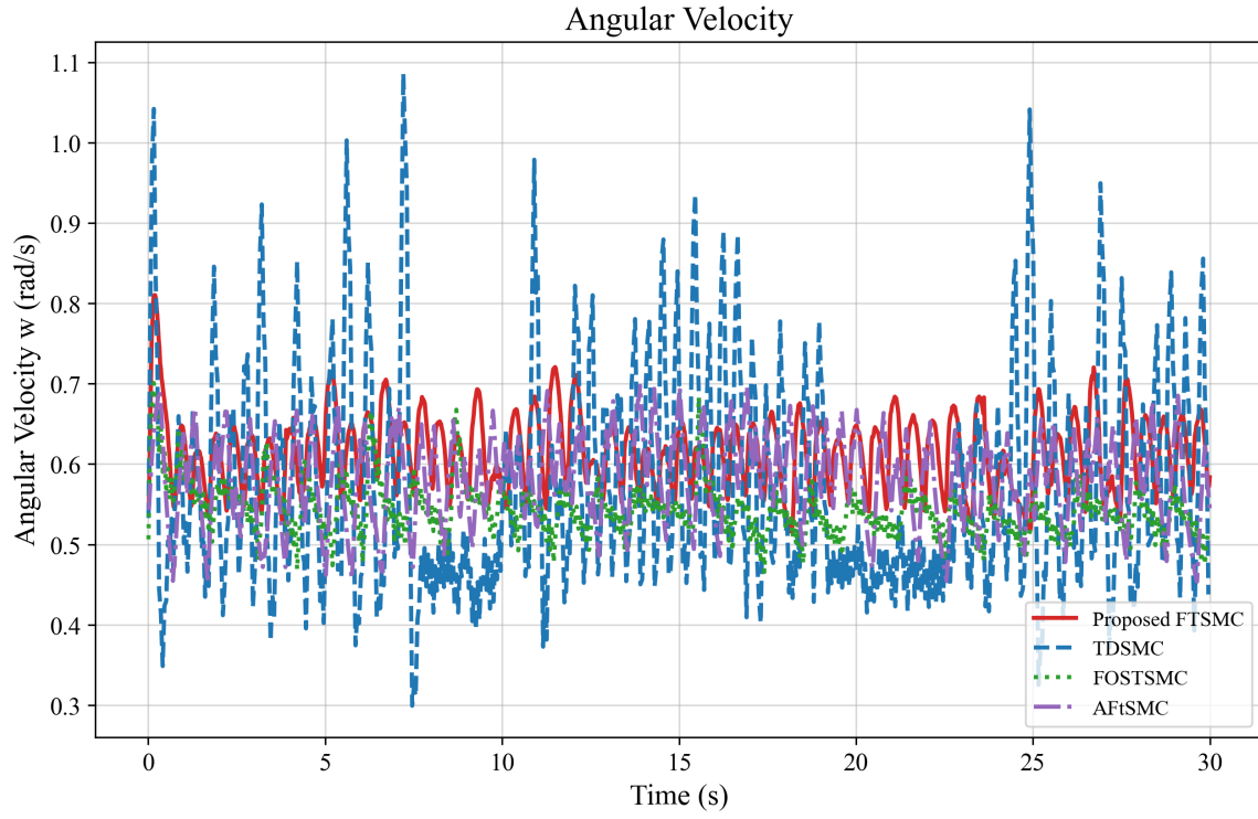
Figure 7. Angular velocity tracking ( \omega_c vs. \omega ) without disturbance.
