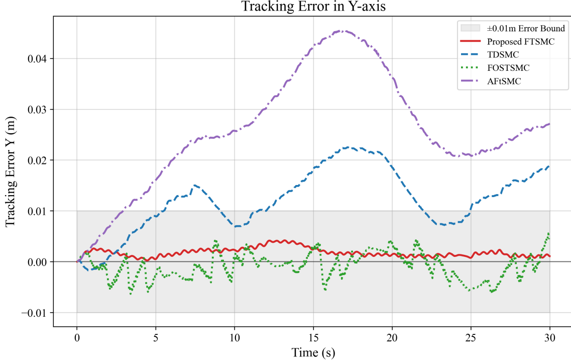
Figure 5. Time evolution of tracking error in Y-axis
