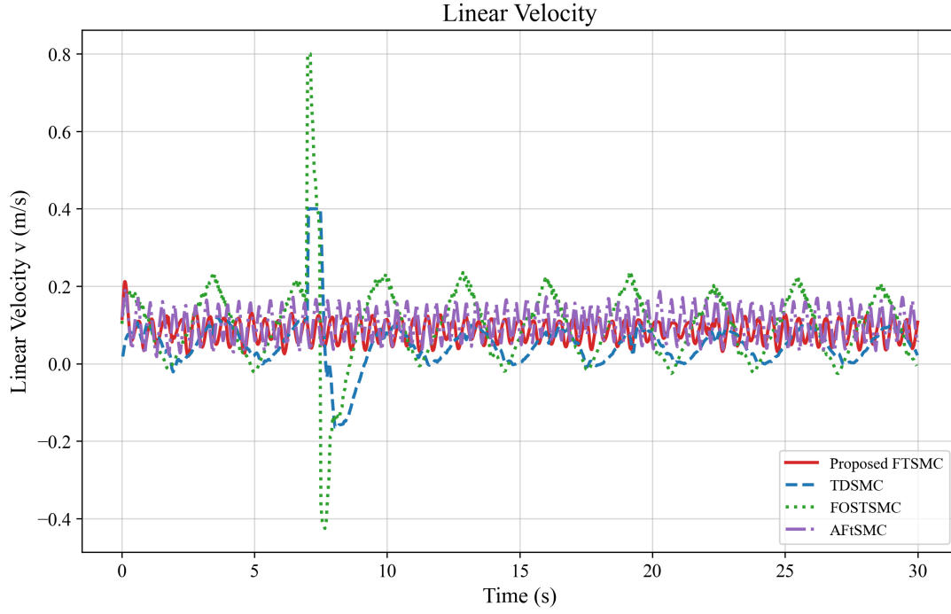
Figure 14. Linear velocity tracking ( v_c vs. v ) with disturbance
