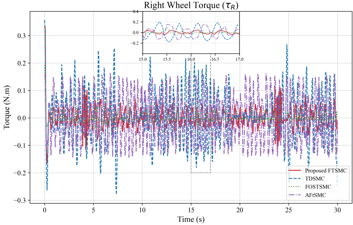
Figure 9. Control input: \tau_R without disturbance
