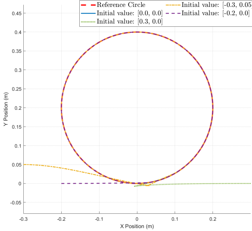
Figure 11. Trajectory tracking performance of the proposed scheme with different initial conditions
