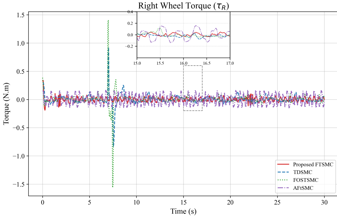
Figure 17. Control input: \tau_R with disturbance
