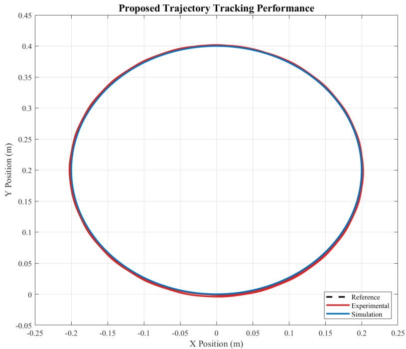
Figure 18. Proposed trajectory tracking performance (simulation and experiment)
