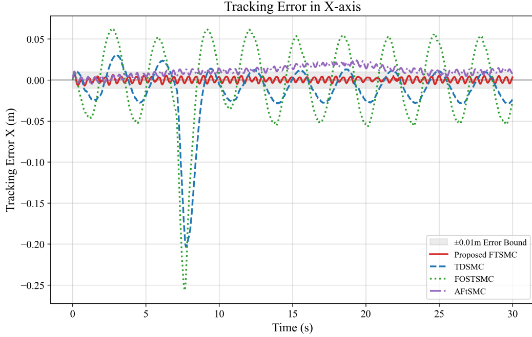
Figure 12. Time evolution of tracking error in X-axis
