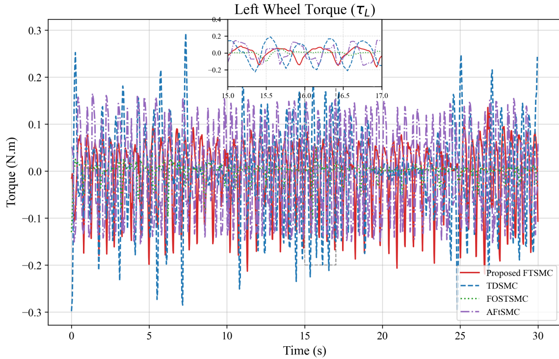
Figure 8. Control input: \tau_L without disturbance
