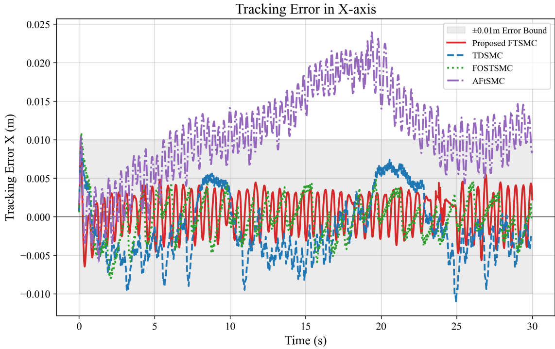
Figure 4. Time evolution of tracking error in X-axis
