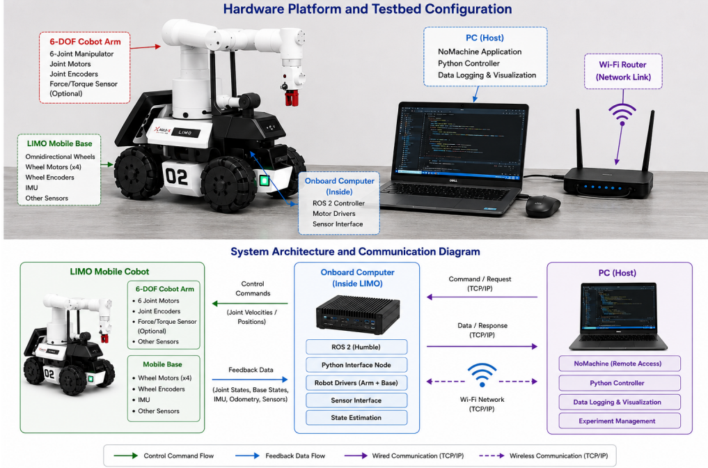
Figure 2. Experimental setup of the LIMO mobile robot platform
