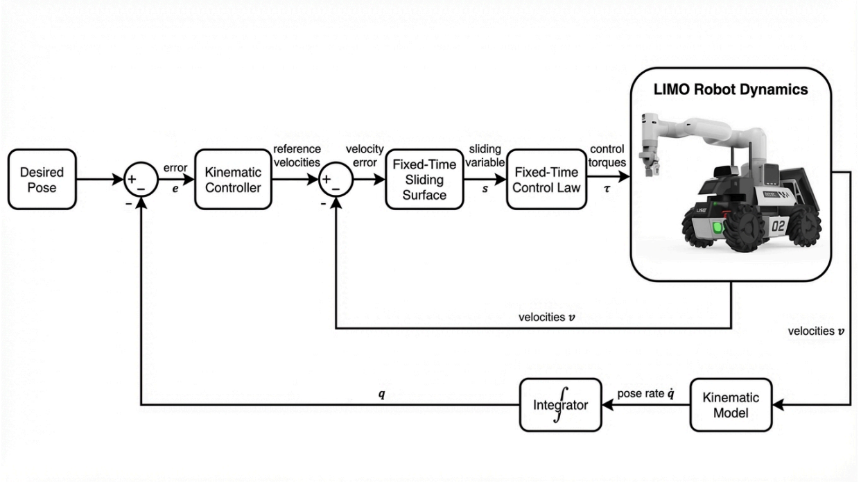
Figure 1. General block diagram of the proposed fixed-time sliding mode control scheme
