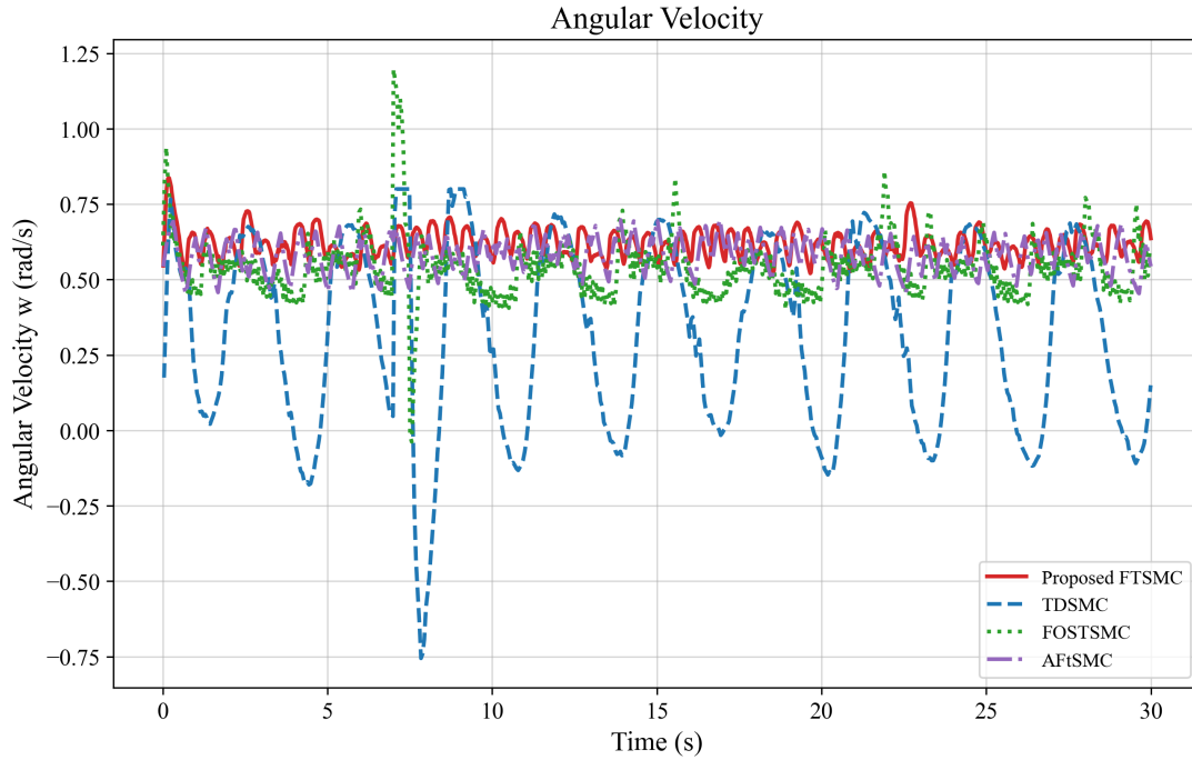
Figure 15. Angular velocity tracking ( w_c vs. w ) with disturbance
