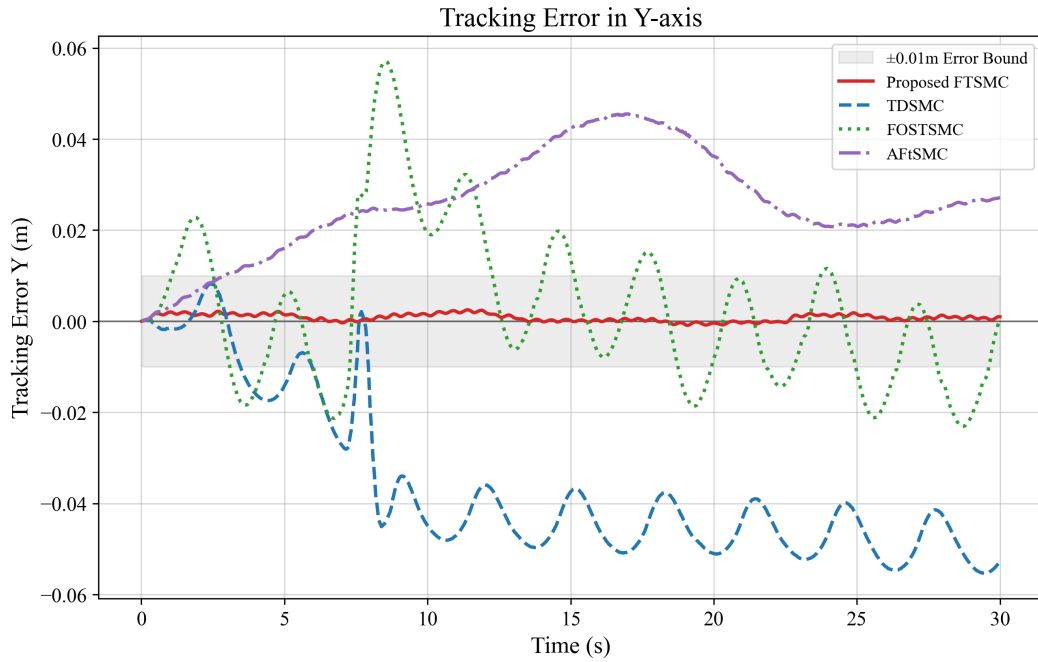
Figure 13. Time evolution of tracking error in Y-axis
