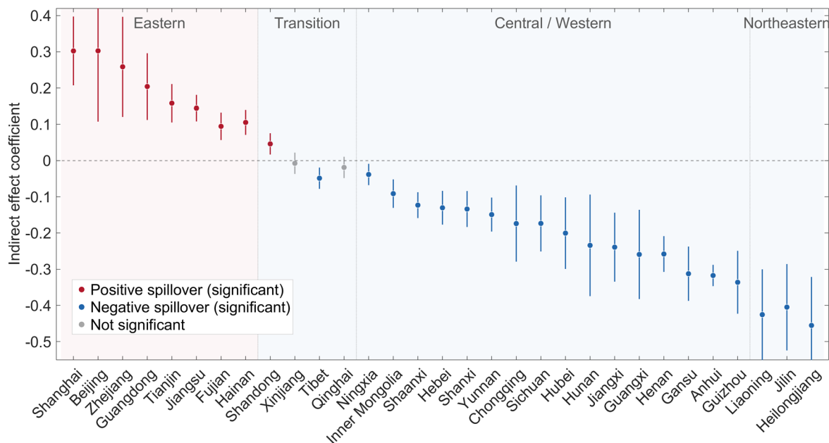
Figure 4. Provincial indirect effects of Net Demographic Dividend Transfer index on old-age dependency ratio from the spatial Durbin model. Error bars represent 95% confidence intervals. Provinces are ordered by indirect effect magnitude.
