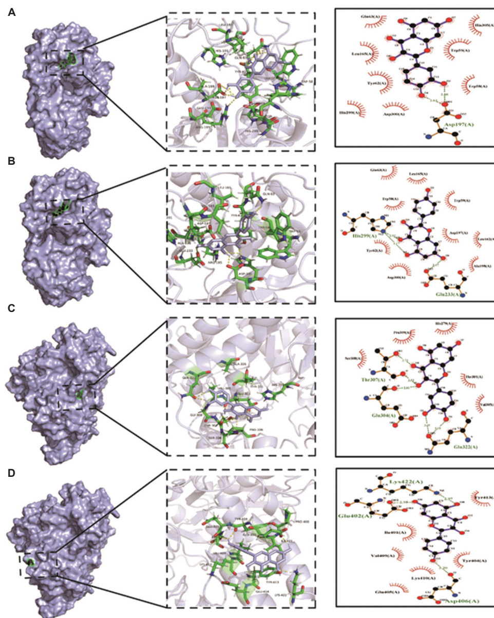
Figure 6. The molecular docking results between quercetin, and kaempferol, and \alpha -amylase/ \alpha -glucosidase. The 3D binding diagram of quercetin- \alpha -amylase (A), kaempferol- \alpha -amylase (B), quercetin- \alpha -glucosidase (C), and kaempferol- \alpha -glucosidase (D) (left), and the corresponding 2D interaction diagrams (right).
