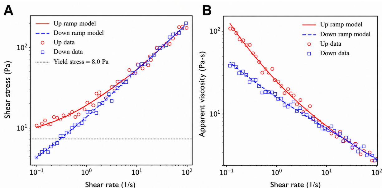
Figure 4. Rheological properties of the antibacterial emulsion system, Emulsion 1. (A) Flow curves displaying shear stress as a function of shear rate for increasing (solid red) and decreasing (dashed blue) ramps, including experimental data. The yield stress, indicated by the horizontal dotted line, demonstrates the critical stress threshold required for flow initiation. (B) Apparent viscosity hysteresis loops showing viscosity versus shear rate during the upward and downward ramps, illustrating the time-dependent breakdown and recovery of the material's internal structure.
