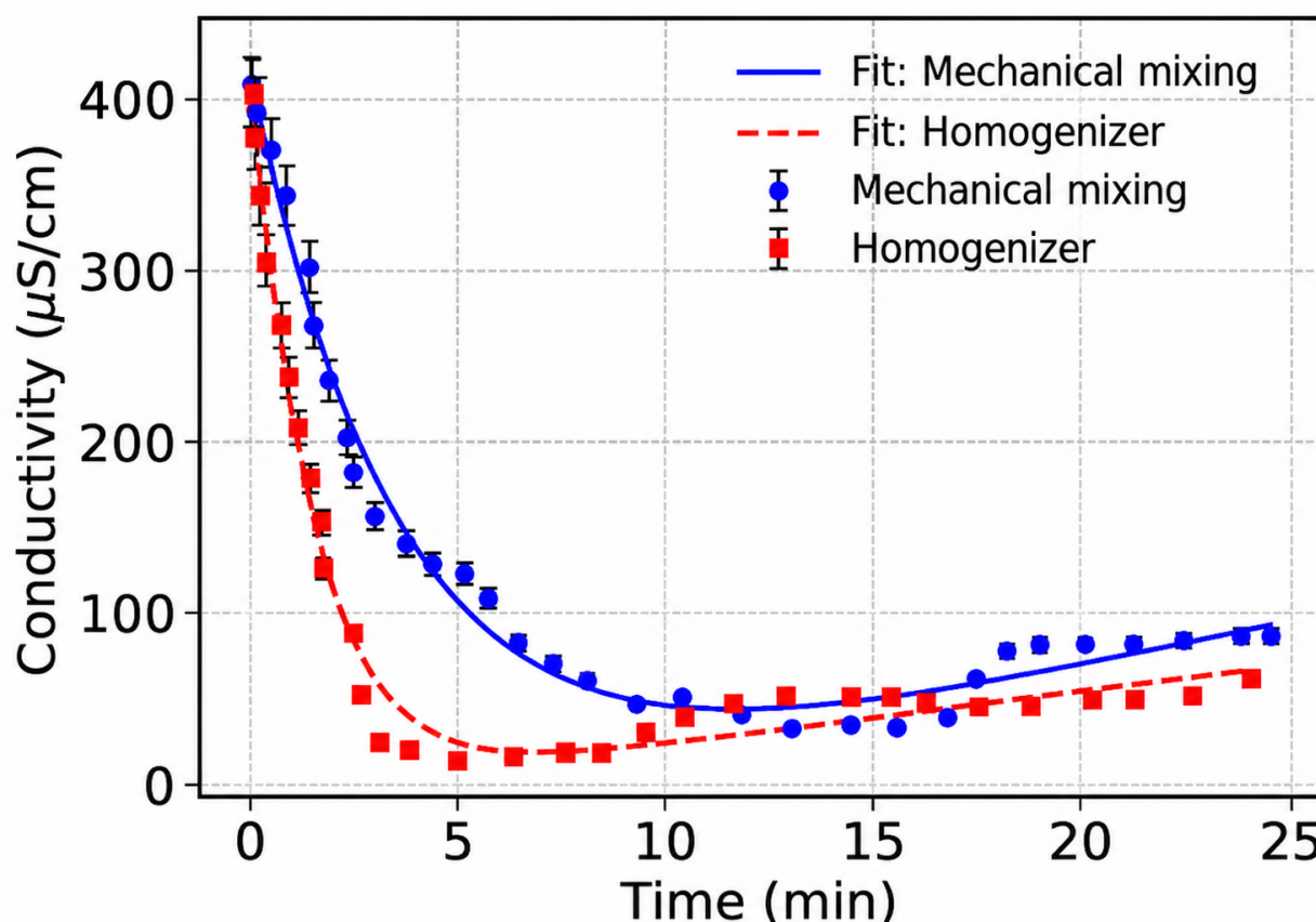
Figure 2. Comparison of conductivity changes over time for mechanical mixing and homogenizer treatments during emulsification. Fits are based on exponential decay plus linear recovery. Error bars represent the range of uncertainty in data collection.
