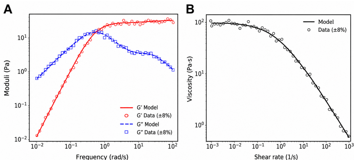
Figure 3. Three percent methyl cellulose solution in water. (A) Frequency-dependent storage modulus ( G' ) and loss modulus ( G'' ) fitted using a two-element Maxwell model. (B) Shear-rate dependent viscosity modeled using the Cross model. In both panels, open symbols represent experimental data.
