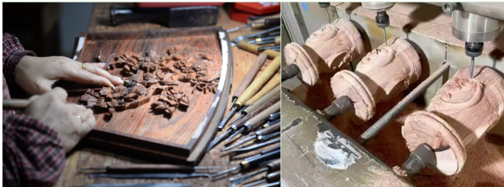
Figure 4. Comparison of hand carving and computer numerical control (CNC) wood carving. Left: hand-carved woodwork showing visible hand-tool marks; right: CNC woodcarving process, which produces more uniform surfaces and lacks the irregular marks characteristic of hand carving. Source: Photos by the authors (2025)
