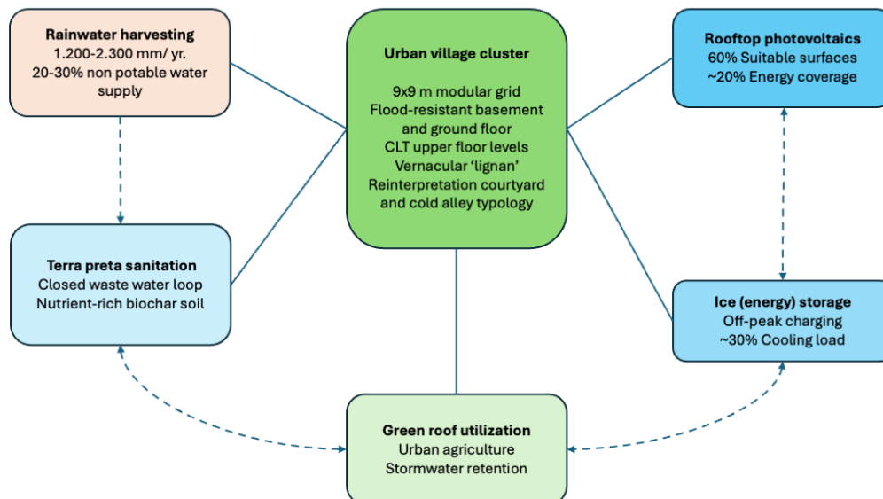
Figure 5. Closed-loop resource cycle diagram illustrating the integration of rainwater harvesting, rooftop photovoltaics, ice energy storage, and Terra Preta sanitation within the cluster framework. Source: Diagram by the authors
