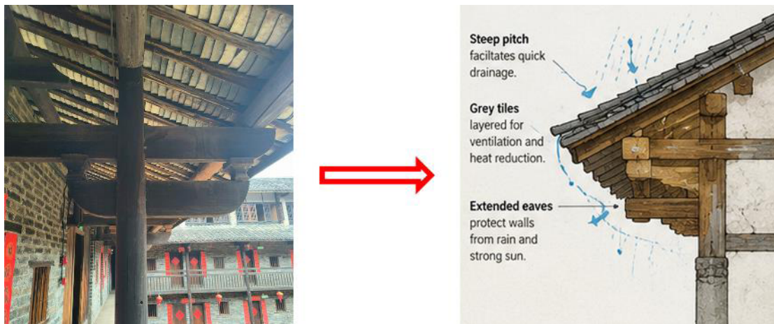
Figure 4. Roof drainage and layered tile roofing structure. Source: Photo and drawing by the authors
