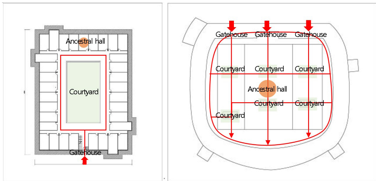
Figure 8. Comparative spatial configuration of Yanyiwei and Wushiwei. This schematic diagram highlights the spatial relationship among the gatehouse, courtyard system, and ancestral hall, illustrating differences in access control, circulation depth, and ritual centrality between the two enclosure types. Source: Drawings by the authors
