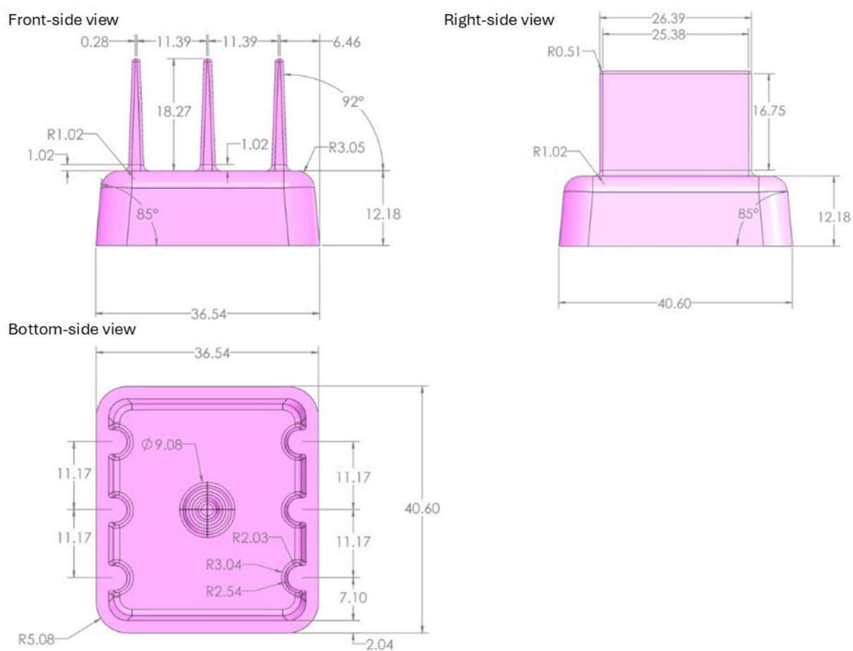
Figure S1. Orthographic projections of the molded part. All dimensions are given in mm
