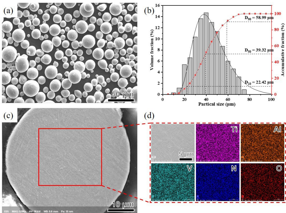
Figure 1. Ti6Al4V powder. (a) Scanning electron microscopy (SEM) image of overall powder morphology. Scale bar: 50 \mu\text{m} ; magnification: 5,000 \times . (b) Particle size distribution. (c) SEM image of a particle cross-section. Scale bar: 10 \mu\text{m} ; magnification: 5,000 \times . (d) Magnified view with energy-dispersive spectroscopy (EDS) mapping showing solute element distribution. Scale bars: 5 \mu\text{m} ; magnifications: 5,000 \times .
